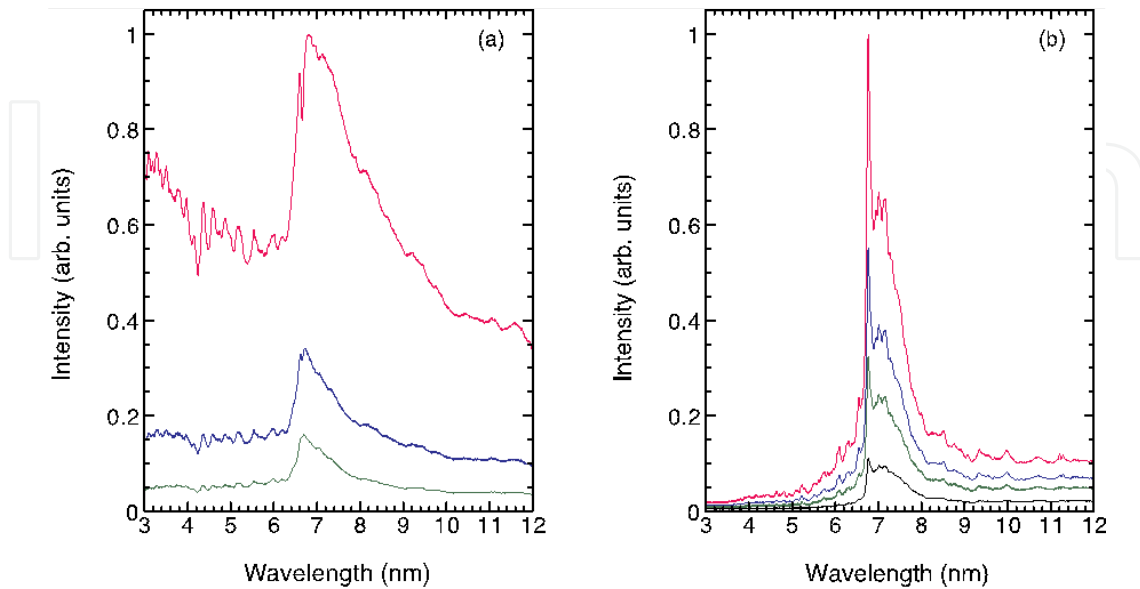
Figure 4. (a) Time-integrated EUV emission spectra from the Nd:YAG LPPs at different laser intensities of 9.7 \times 10^{11} , 2.2 \times 10^{12} , and 6.6 \times 10^{12} W/cm 2 , respectively. The peak wavelength shifts from 6.7 to 6.8 nm with increasing the laser intensity. (b) Time-integrated EUV emission spectra from the CO 2 LPPs at different laser intensities of 5.5 \times 10^{10} , 8 \times 10^{10} , 9.8 \times 10^{10} , and 1.3 \times 10^{11} W/cm 2 , respectively. The peak wavelength of 6.76 nm remains constant with increasing the laser intensity [14].
