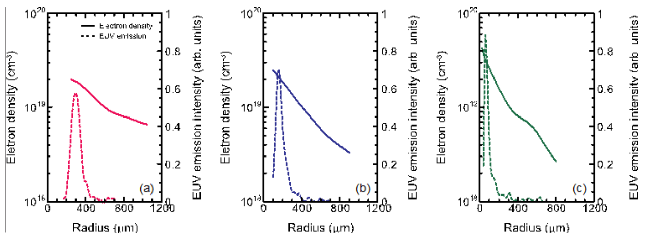
Figure 3. Profiles of the radial electron density (solid line) and radial EUV emission (dashed line) at the time of three different peak laser intensities of (a) 1 × 10 12 W/cm 2 , (b) 7 × 10 12 W/cm 2 , and (c) 1 × 10 14 W/cm 2 , corresponding to laser focal spot and target diameters of (a) 500 μm, (b) 200 μm, and (c) 50 μm [22].
