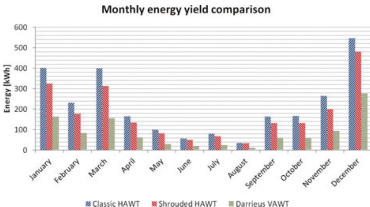
Figure 8. Monthly energy output for the chosen turbines [23].
