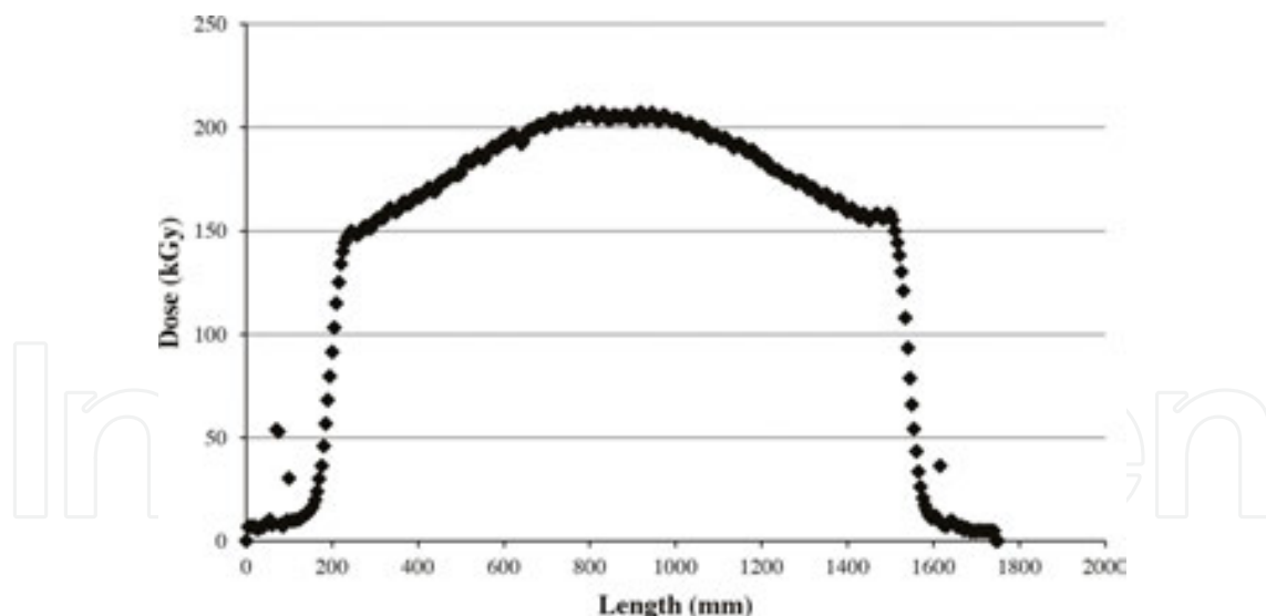
Figure 2. Dose along the sludge delivery system. The measurements were taken using cellulose triacetate film irradiated with 3 MeV electrons, 15 mA of current, 5 s of exposure time and 100% scanning aperture [7].
