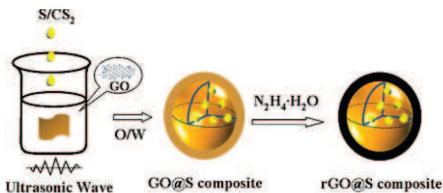
Figure 16. Schematic of synthesis steps for S@rGO composite [42].
