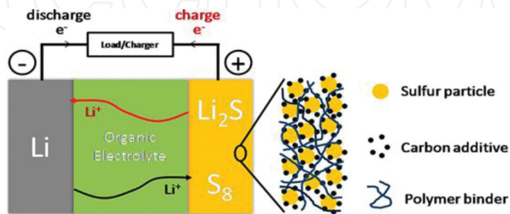
Figure 2. Structure scheme of Li-S battery [11].
