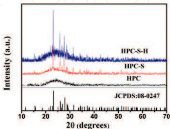
Figure 8. XRD patterns of the as-prepared core-shell HPCs, HPCs-S-H and HPCs-S composite [28].
