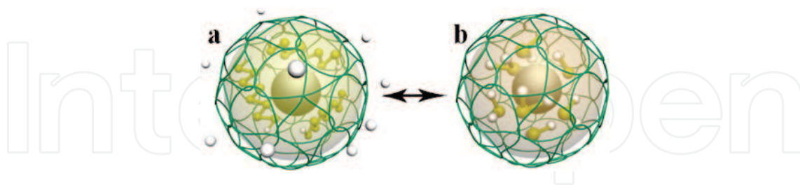
Figure 26. \text{Li}_2\text{S} (orange color) trapping within the PANI framework during lithiation/delithiation (yellow and gray are the sulfur and lithium) [47].
