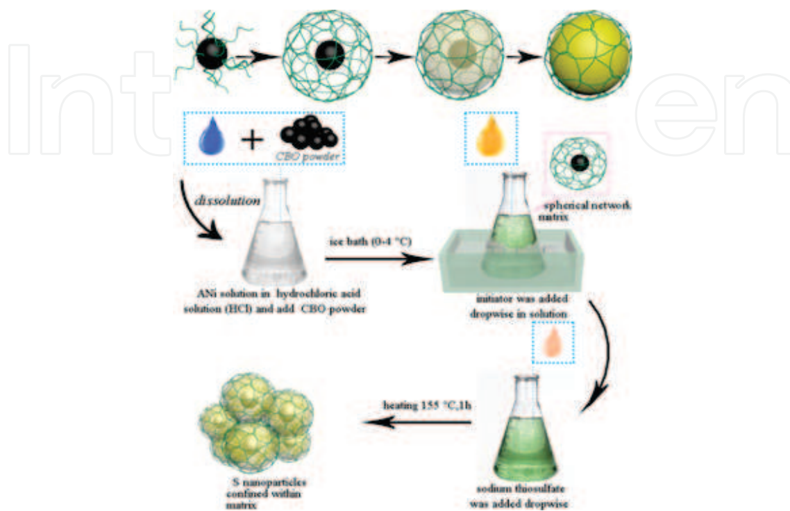
Figure 22. The design of PSN matrix (C-S@PANI composite) as the cathode materials for lithium-sulfur batteries (Green: PANI, yellow: sulfur, black: acetylene black), and schematic illustration of the synthesis process [47].
