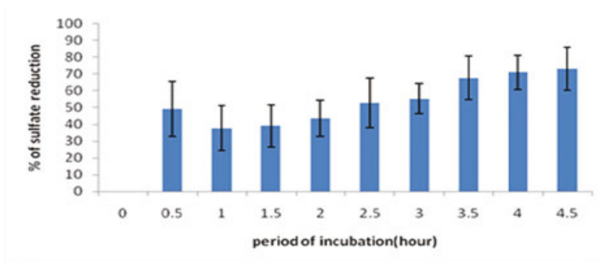
Figure 7. Time course of sulphate reduction by the packed bed bioreactor.
