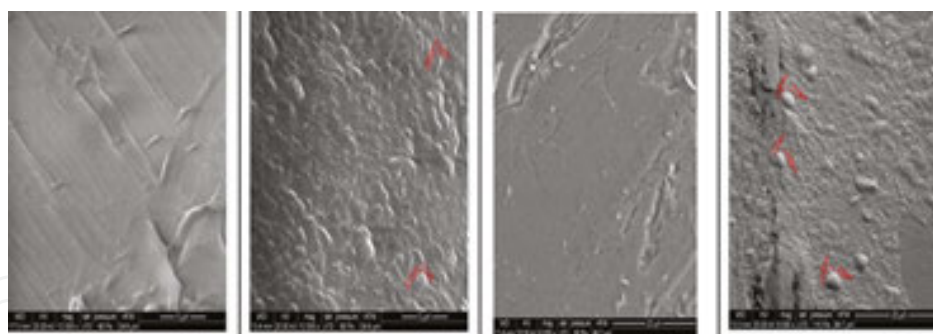
Figure 2. Scanning electron microscopic image of different matrix with and without SRB biofilm. From extreme left, polypropylene matrix (without biofilm), polypropylene matrix (with biofilm), steel matrix (without biofilm), and steel matrix (with biofilm).
