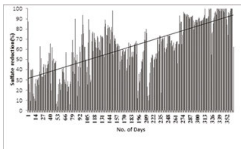
Figure 4. Performance of the SRB consortia in 78-litre packed bed bioreactor for 361 days. The 78-litre bioreactor is constructed of acrylic body and stainless steel for the bottom portion with three nozels for sample collection (distance between first and second nozels is 18 cm, whereas the distance between second and third nozels is 40 cm. The anaerobicity was mentioned by purging nitrogen gas ( 60 \text{ lm/cm}^2 ) into the bioreactor from outside.
