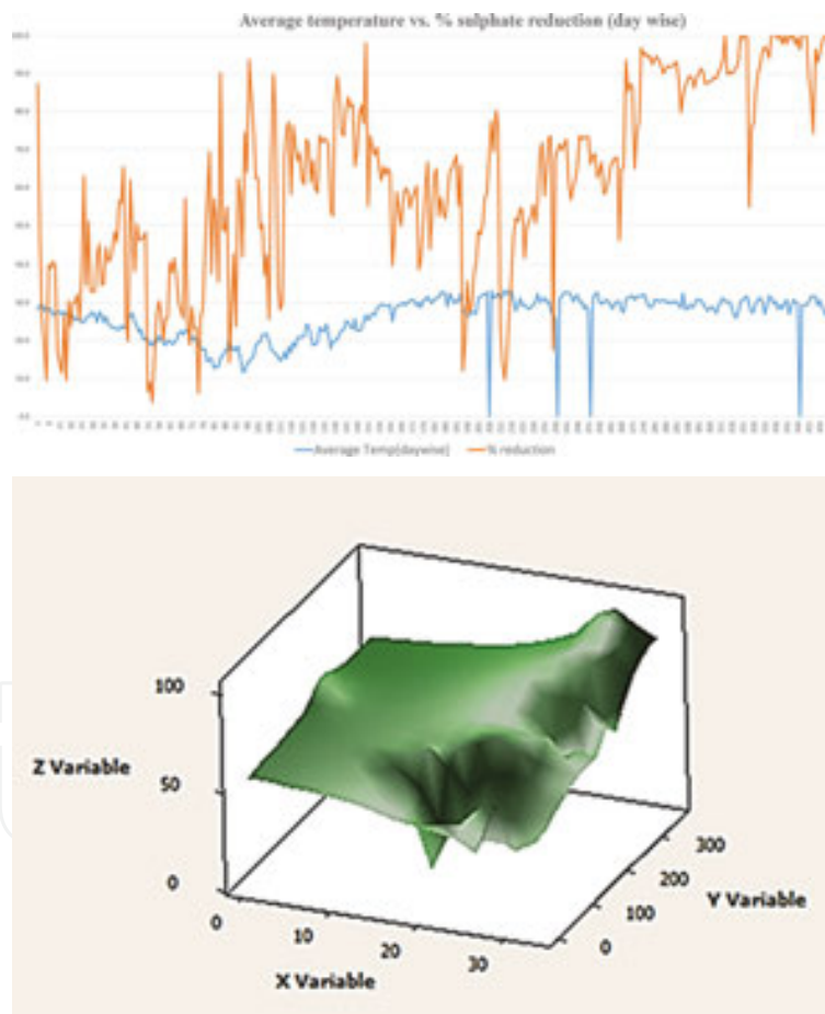
Figure 6. (a) Graph representing biofilm performance in term of sulphate reduction and temperature variation with days. Sulphate reduction indirectly indicates the active biofilm at any point of time. X axis represents days that the reactor was functioning, whereas Y axis represents performance of the system in terms of sulphate reduction in orange colour and ambient temperature in blue. (b) Surface plot among X, Y and Z variables, where Z variable is the percent sulphate reduction, Y variable is the age of the biofilm in days and X variable is the ambient temperature in degree centigrade.
