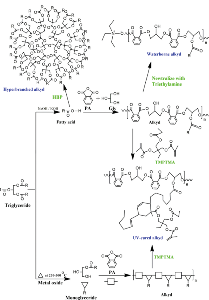
Figure 1. Alkyd synthesis, where R=fatty acid chain (saturated or unsaturated). Where PA:Phthalic anhydride, Gly:Glycerol and TMPTMA: Trimethylolpropane Trimethacrylate.
