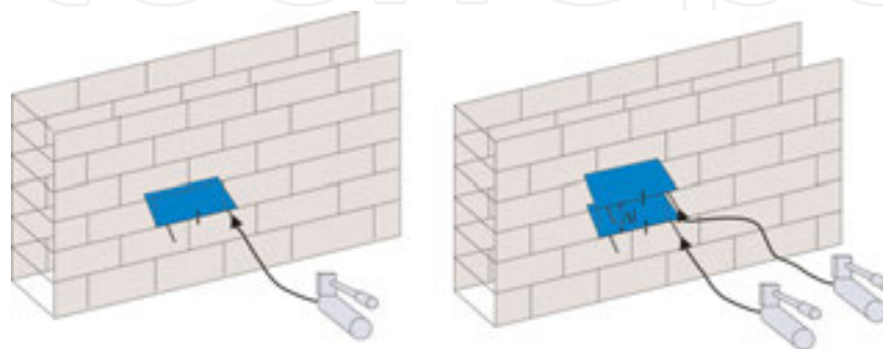
Figure 3. Simple and double flat jack techniques.
