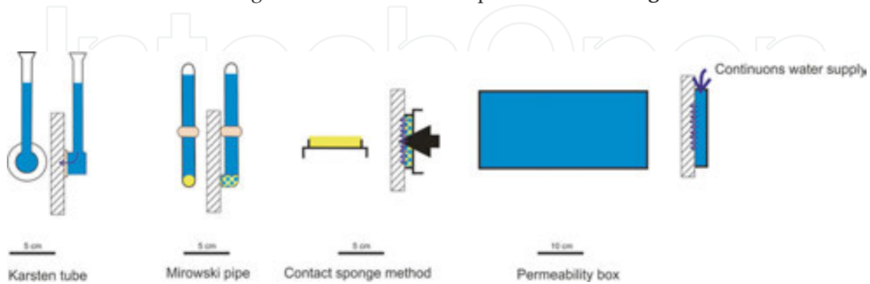
Figure 4. Different systems to measure water absorption “in situ”.
