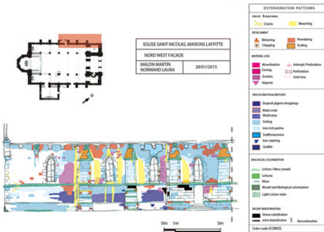
Figure 2. Mapping of weathering types of the Saint Nicolas church at Maisons-Laffitte (France).
