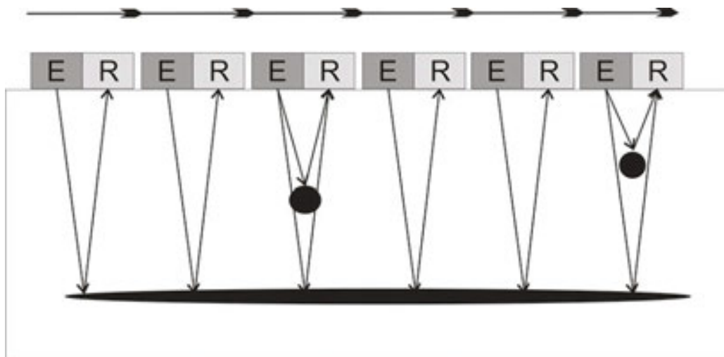
Figure 18. Principle of ground penetrating radar (GPR).
