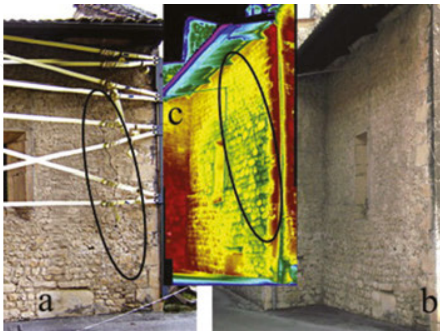
Figure 10. Passive thermography applied to the detection of cracks. (a) Lateral wall of the Church of Santa Maria ad Cryptas (Italy) after the 2009 earthquake; (b) aspect in 2007; (c) thermography image taken in 2007 showing traces of incipient splitting of the masonry. [59].
