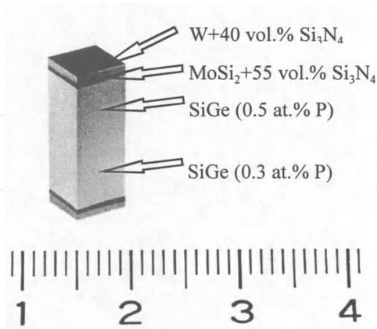
Figure 7. A dense, graded n-type (SiGe) conversion unit produced by HIP [81].
