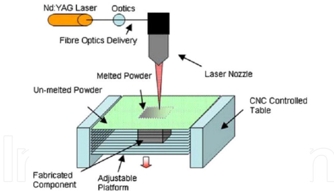
Figure 3. Experimental setup used for laser assisted processing using an Nd:YAG laser power source [55].
