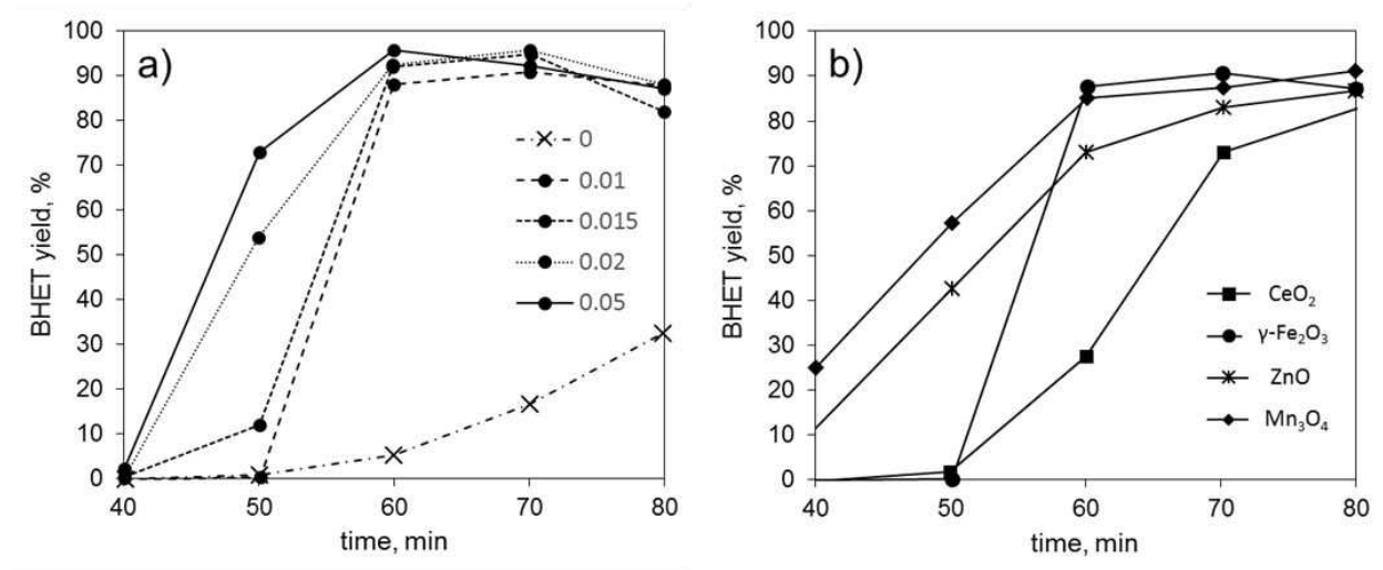
Figure 12. Catalytic performance of \gamma - \text{Fe}_2\text{O}_3 nanoparticles at various loadings and comparison to other metal oxide catalysts. Figure from [12].
