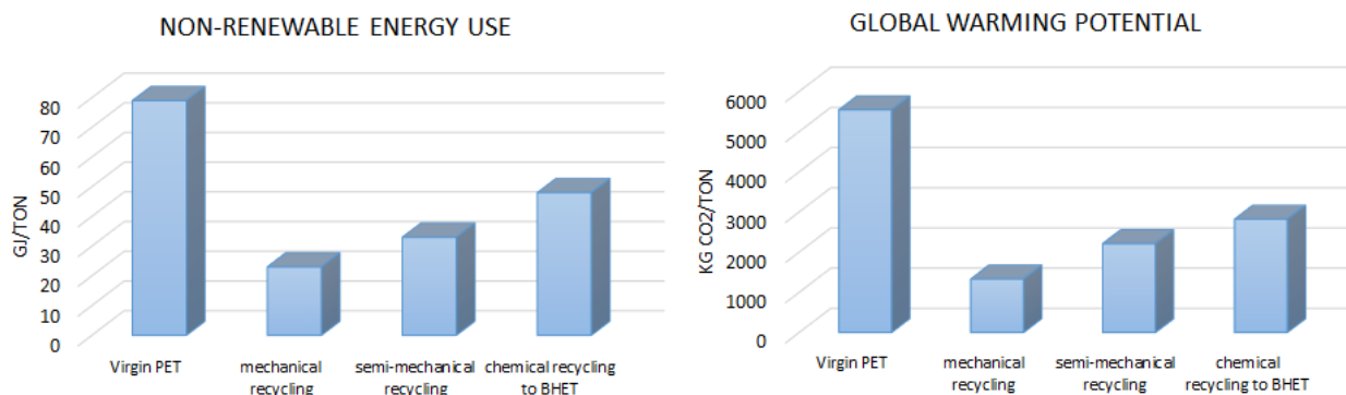
Figure 4. Comparison of life cycle assessment (LCA) results for PET manufacture and recycling in terms of non-renewable energy use and equivalent CO 2 generated per ton of PET fiber [4].
