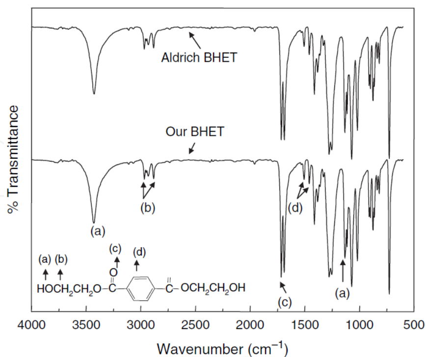
Figure 6. Comparison of FT-IR spectra of standard BHET and BHET recovered from catalyzed glycolysis. Figure from [10].
