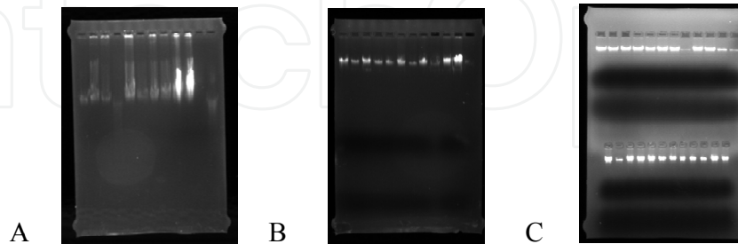
Figure 1. DNA from blood samples. Smeared DNA bands (A), DNA with double-strand breaks (B) and normal intact DNA bands (C). First Report and Final Report of a research grant awarded to Dr. Ivo Sirakov, 2007–2008 – Medicine and Biotechnology – Aids and infectious diseases, Transmissible Spongiform Encephalopathies, funded by the World Federation of Scientists, Geneva, Switzerland.
