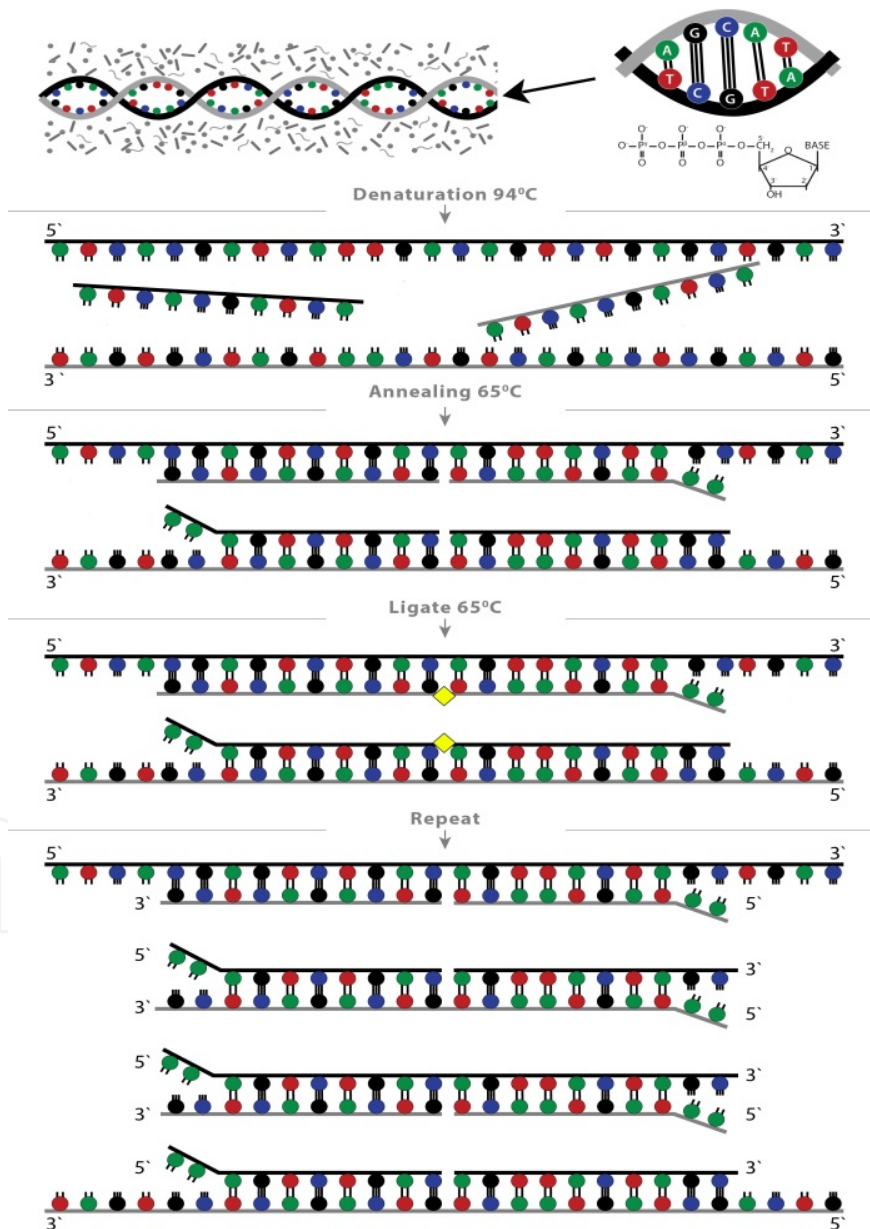
Figure 4. Ligase chain reaction (LCR).
