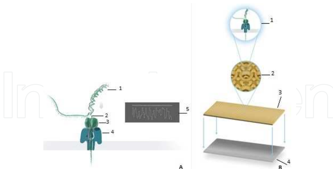
Figure 6. (A) Underlying principle used in nanopore technology sequencing (illustrative data). 1 – DNA library is prepared; 2 – the dsDNA strands are separated and one of the strands passes through 3 – a processive exonuclease enzyme, and 4 – a protein nanopore, in a base-by-base manner, causing a characteristic disruption in the electrical current flowing through the nanopore, which is in fact the signal that is detected in real time. When the end of the first strand is reached, the 3'- to 5'-end hairpin ligation of the two DNA strands allows the processive enzyme to simply continue to push the second strand through the nanopore; 5 – Representative image of DNA sequencing data. (B) 1 – A nanopore protein; 2 – Array of Microscaffold; 3 – Array Chip; 4 – Application Specific Integrated Circuit.
