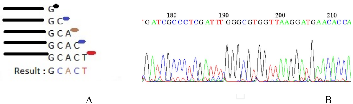
Figure 5. Generation of fragments by incorporation of dNTPs and ddNTPs (labeled) in the Sanger method and cycling sequencing (A). Sample electropherogram (portion) of the beta-lactamase OXA-48 gene of Klebsiella pneumoniae strain OXA48BG, NCBI, GenBank accession number KJ959619.1 [54] (B).
