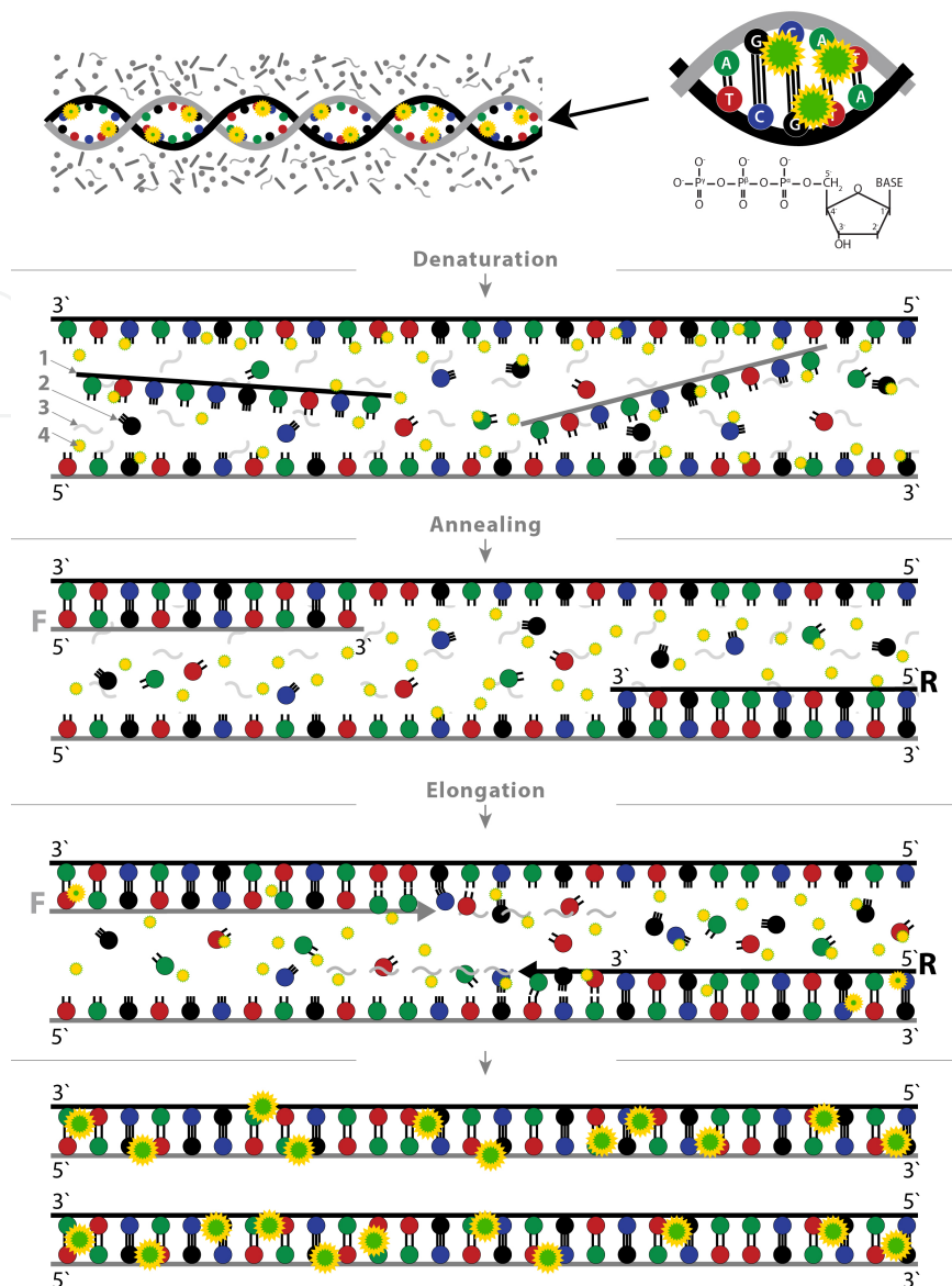
Figure 2. Polymerase chains reactions (PCRs). Components of reactions: 1 – Primers forward and reverse; 2 – deoxynucleoside triphosphates - dATPs, dGTPs dCTP, and dTTPs; 3 – Taq polymerase; 4 – probe labeled with reporter (R) and quencher (Q) molecules; 5 – SYBR Green dye; (A) Conventional PCR includes the following steps: an elongation cycle at 95°C for 1–5 min to activate the polymerase → DNA or cDNA denatures (melts) at 95°C → complementary sequences with specific melting temperature anneal to each other at 40–65°C for 30–120 s → nucleotides are incorporated in the growing strand and the target sequence is amplified at 72°C for up to 60 s. After 35 cycles, a single dsDNA copy is amplified into 2 36 copies; (B) TaqMan real-time PCR (real-time PCR Taq has 5′–3′ exonuclease activity) 3(b) underlying principle of TaqMan real-time PCR. The reaction mixture includes the same main components as conventional PCR plus a synthetic oligonucleotide (probe) that is labeled with a reporter and a quencher and is complementary to an internal region in the 3′–5′ strand of the sequence of interest (4). The reaction can also include two steps per cycle – denaturation at 95°C and annealing/elongation at 60°C [8, 45]; and (C) Underlying principle of SYBR Green real-time PCR. SYBR Green dye (5) non-specifically binds to dsDNA. During denaturation, the dye is released; it then binds again to the PCR fragment during the elongation step. SYBR Green emits fluorescence when bound to dsDNA. Thus, the more fragments are amplified, the stronger the fluorescence intensity will be. The signal is graphically recorded the same way as in the TaqMan reaction.
