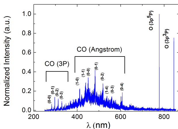
Figure 3. Appearance of the emission spectrum of a pure CO 2 microwave discharge acquired at Z=7\text{ cm} . The notation ( v'-v'' ) refers to the vibrational transition, where v' ( v'' ) stands for upper (lower) vibrational energy level. Reproduced with permission from Ref. [20]. Copyright 2014 IOP Publishing.
