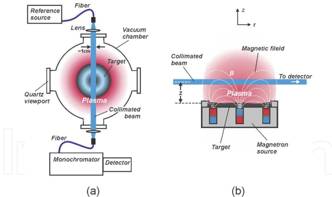
Figure 5. Top (a) and side (b) view of the experimental setup utilized for absolute density measurements in a magnetron sputtering discharge by ROAS. Role of the reference source is played by a hollow cathode lamp. Reproduced with permission from Britun et al. [38]. Copyright 2015 AIP Publishing.
