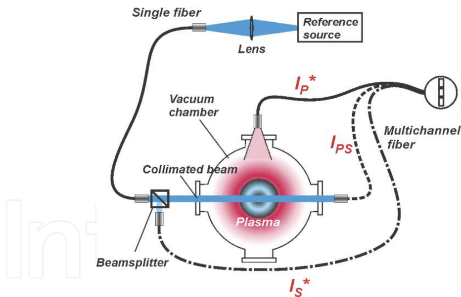
Figure 6. Scheme of the experimental setup for absorption measurements with increased reliability utilizing simultaneous acquisition of the plasma and source optical signals ( I_P , I_S , and I_{PS} ) necessary for calculation of the line absorption A_L .
