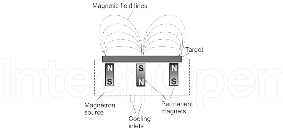
Figure 1. Side view of a typical magnetron source, including planar circular magnetron target, permanent magnets, and cooling system. The magnetic field lines are shown schematically.
