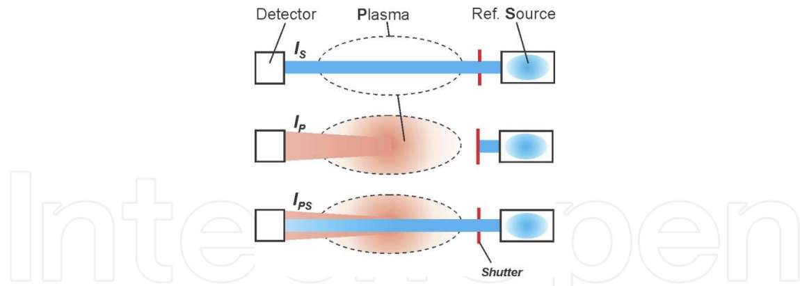
Figure 3. Schematic illustration of the absorption technique and the physical meaning of the quantities I_p , I_s , and I_{PS} .
