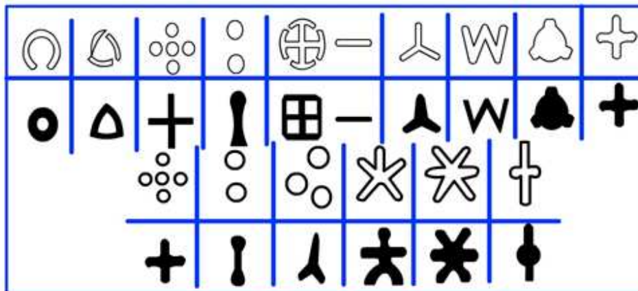
Figure 4. Cross-sectional View of Polyester Fibers [23]
