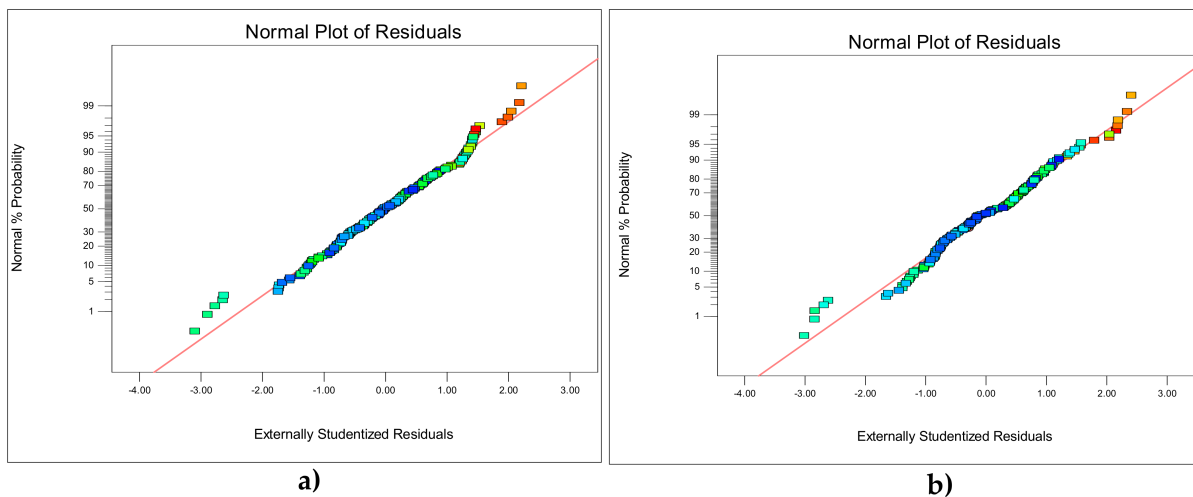
Figure 15. Normal Plot of Residual Coefficient of Friction Values: (a) Static and (b) Kinetic
