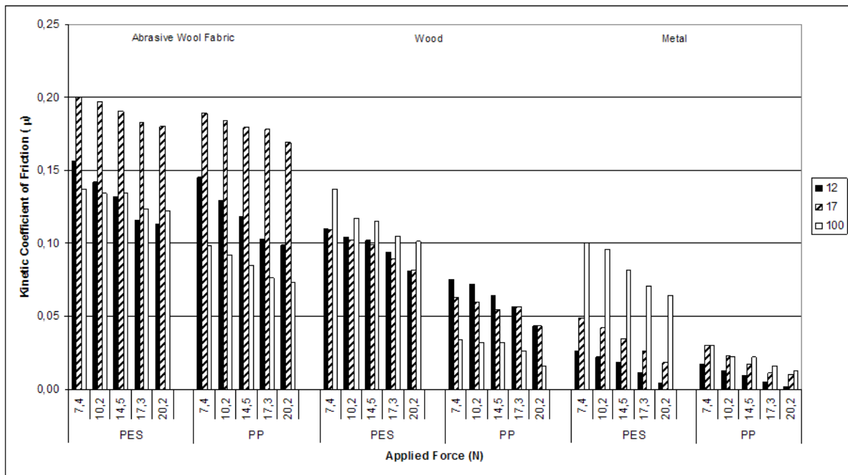
Figure 13. MD Kinetic Friction Coefficient
