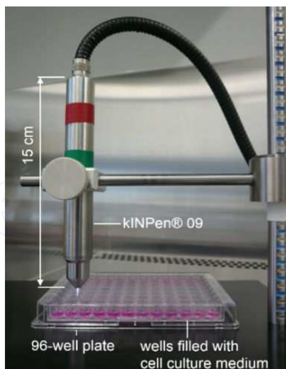
Figure 1. Experimental setup for argon plasma treatment of cell culture media. The kINPen®09 was mounted vertically. The distance between the tip of the quartz capillary and the 96-well plate does not exceed 1 mm.
