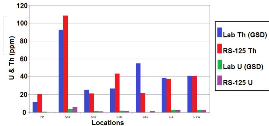
Figure 5. Correlation of RS-125 to laboratory assays for Leeuwin Complex samples.
