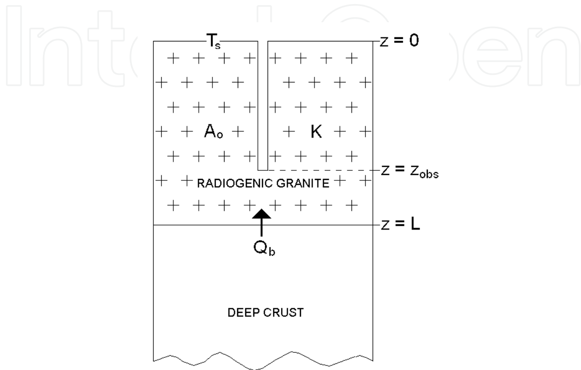
Figure 3. theory for temperature model. Note that the same modeling geometry is used for relatively thin enrichment layer models in section 7. In the latter case, the radiogenic granite layer is a layer where U- and Th-rich fluids have been rapidly emplaced due to chemical alteration processes, largely due to weathering and erosion.
