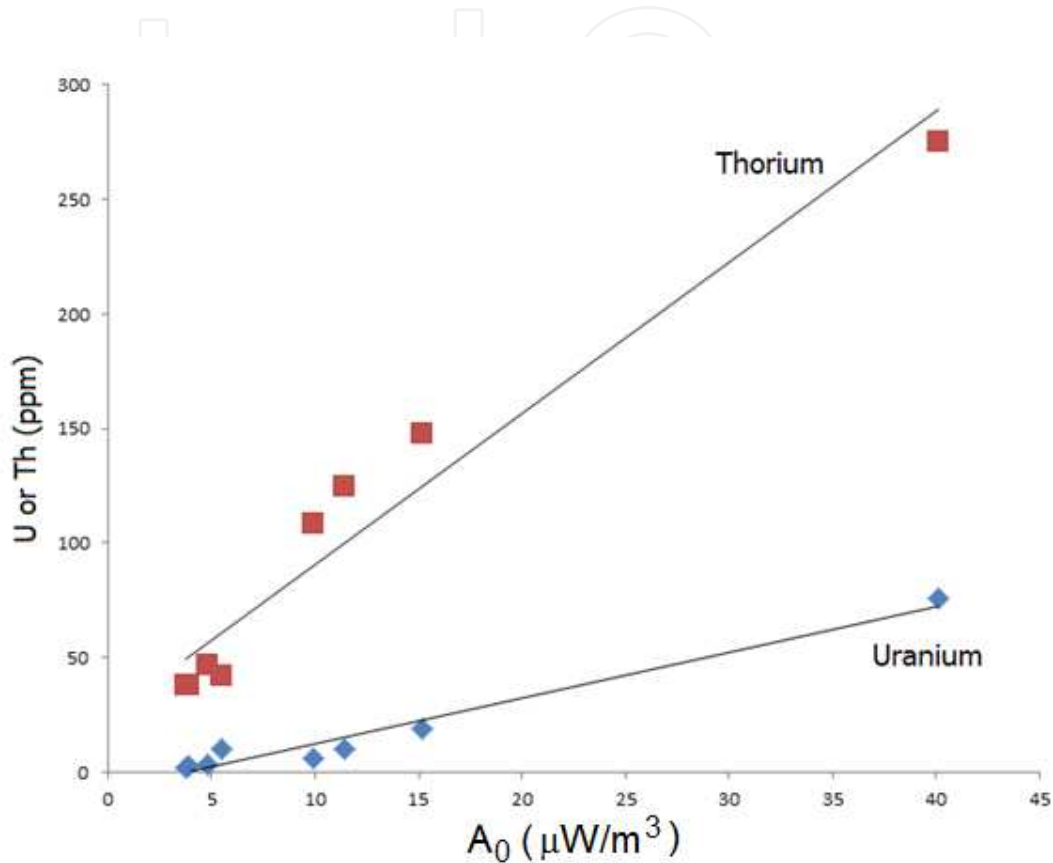
Figure 7. Correlation of U or Th concentration to heat generation, using Eq. (4).
