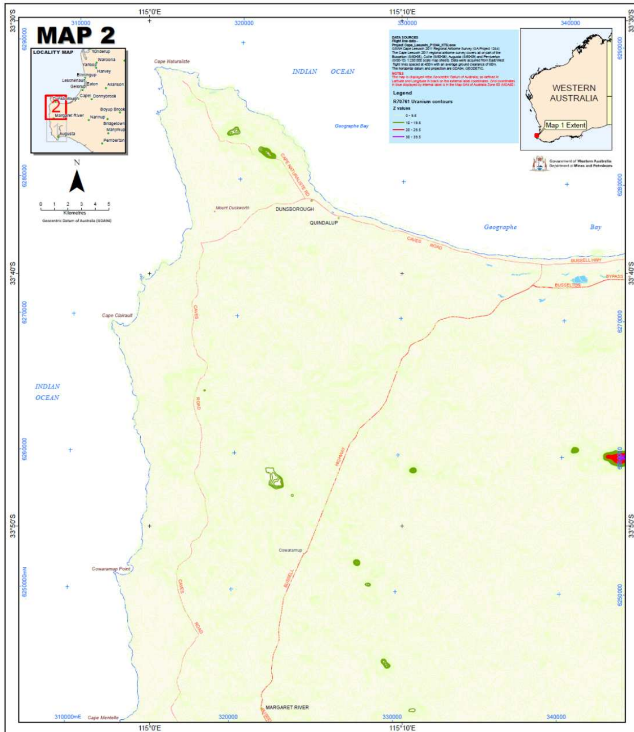
Figure 10. Uranium distribution in Dunsborough region (GWA database).
