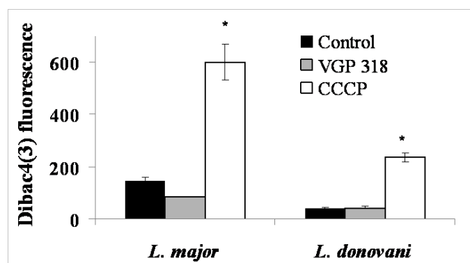
Figure 5. Compound VGP-318 does not alter the plasma membrane potential in Leishmania lines. Promastigotes were incubated with 30 μM of compound VGP-318 for 3 h and then treated with 2 μM of the specific plasma membrane potential probe DIBAC4(3) for 10 min at 28 °C. Untreated parasites were used as control, and treatment with 10 μM CCCP was used as 100% depolarization of the plasma membrane potential. Data are means ± SD of three independent experiments. Significant differences were determined using Student's t -test (* p < 0.01).
