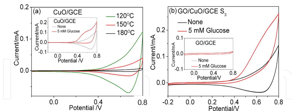
Figure 9. CV curves of (a) CuO NPs synthesized at 120, 150, and 180°C. The inset is the CuO NPs synthesized at 120°C in 0.1 M NaOH before (black trace) and after (red trace) the injection of 5 mM glucose. (b) CuO/GO composite S3 and GO sheet (inset) in 0.1 M NaOH before (black trace) and after (red trace) the injection of 5 mM glucose. (Reproduced with permission from ref. 16. Copyright ACS 2013)
