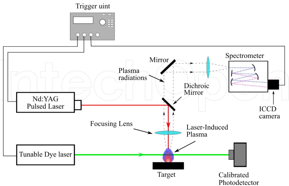
Figure 4. Schematic illustration of a combined set-up of laser-induced fluorescence and optical emission spectroscopy of laser-induced plasma
