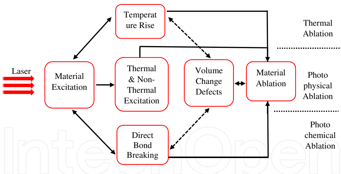
Figure 3. Graphical illustration of mechanisms leading to pulsed laser ablation
