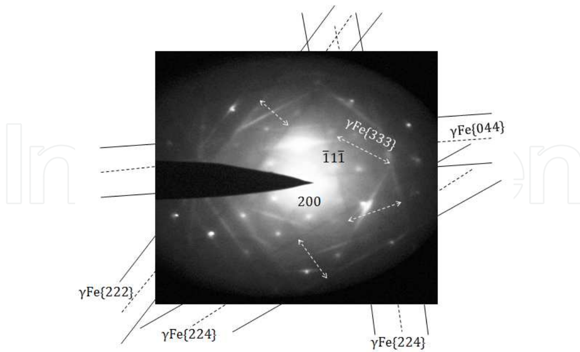
Figure 8. The spots, Kikuchi lines and the distance between paired Kikuchi lines in the pattern of \gamma Fe are determined.
