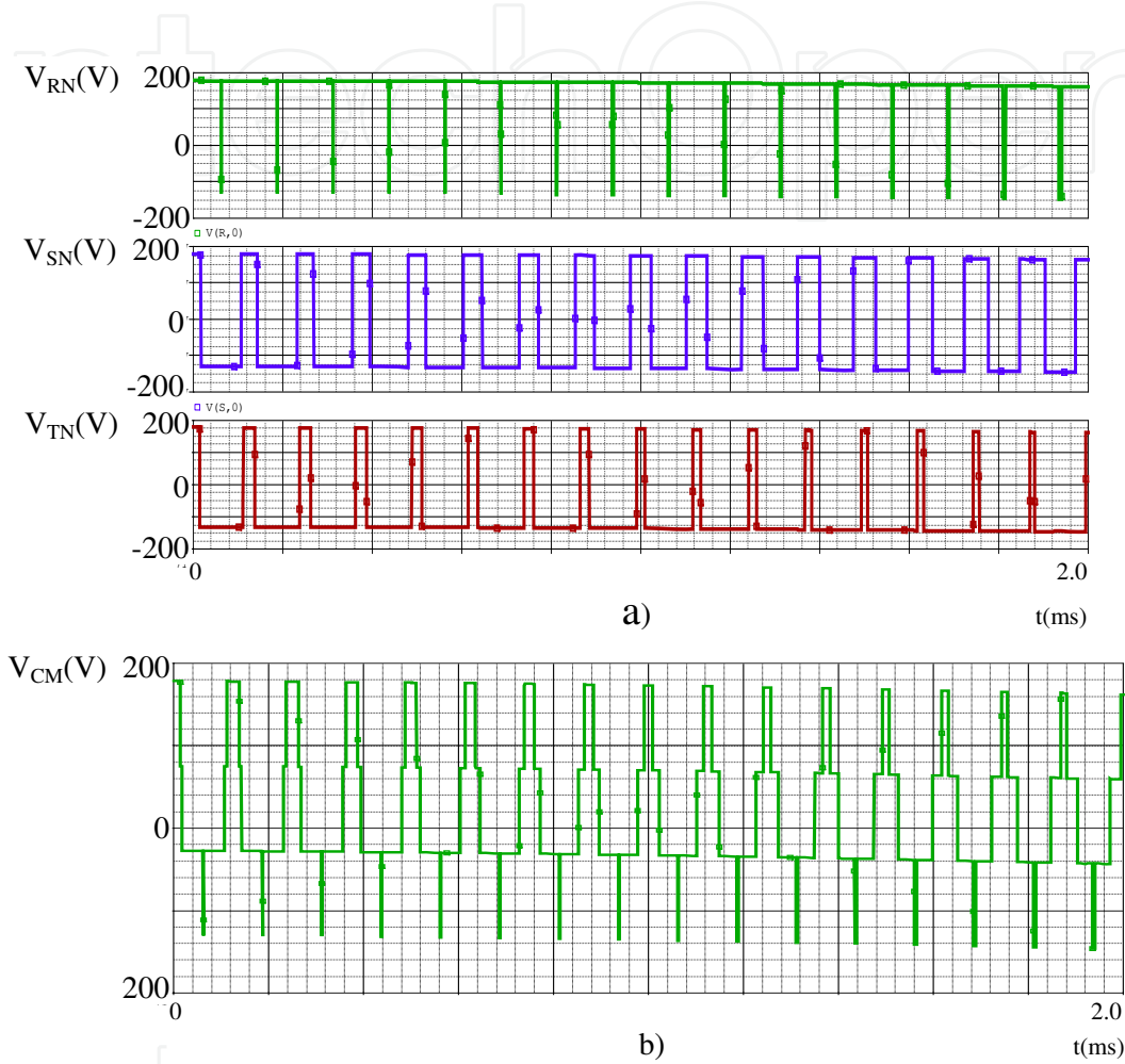
Figure 7. a) Phase voltage, b) a common mode voltage ( V_{CM} ) - f_s = 16 kHz
