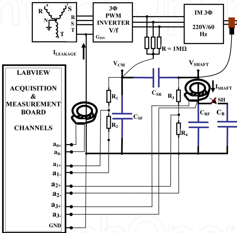
Figure 10. Measuring circuit of the quantities of interest
