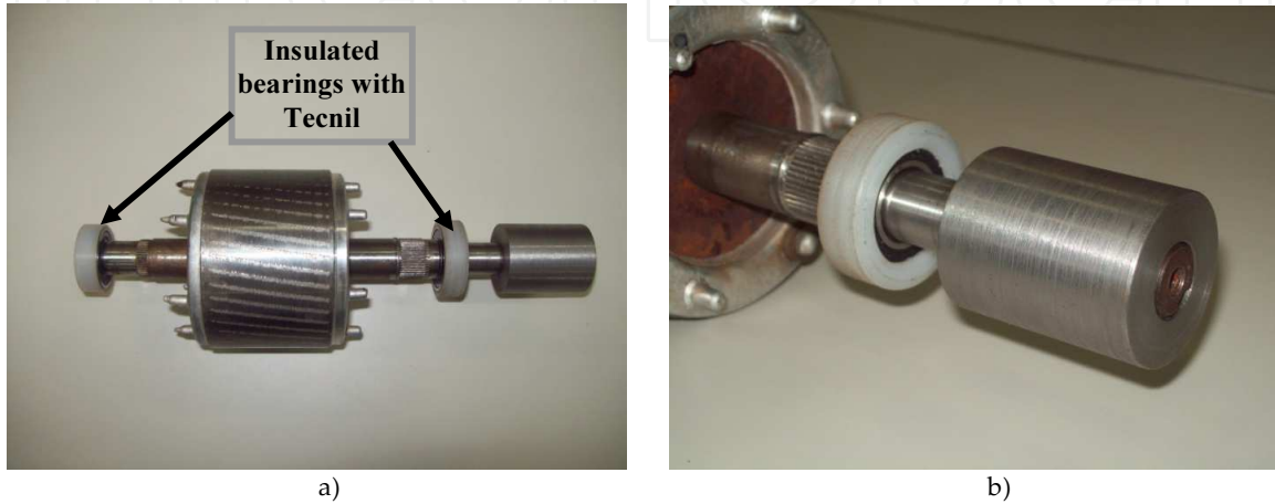
Figure 11. a, b): Insulation of the motor shaft bearings
