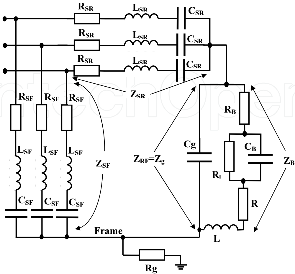
Figure 1. High-frequency equivalent circuit of induction motor
