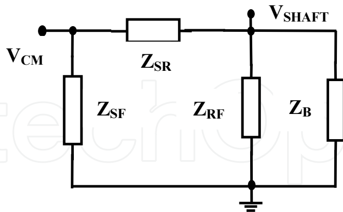
Figure 2. High-frequency simplified circuit for three-phase induction motor according to its impedances
