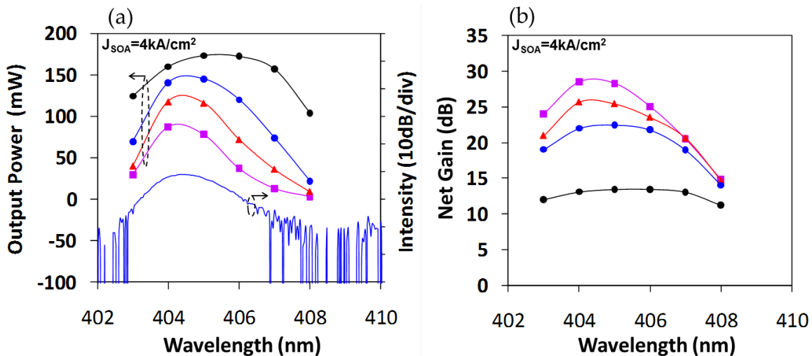
Figure 8. (a) Output power and ASE spectra and (b) net gain spectra obtained from device A at input powers of 11 \text{ mW} (black), 1.2 \text{ mW} (blue), 0.4 \text{ mW} (red), and 0.2 \text{ mW} (violet).
