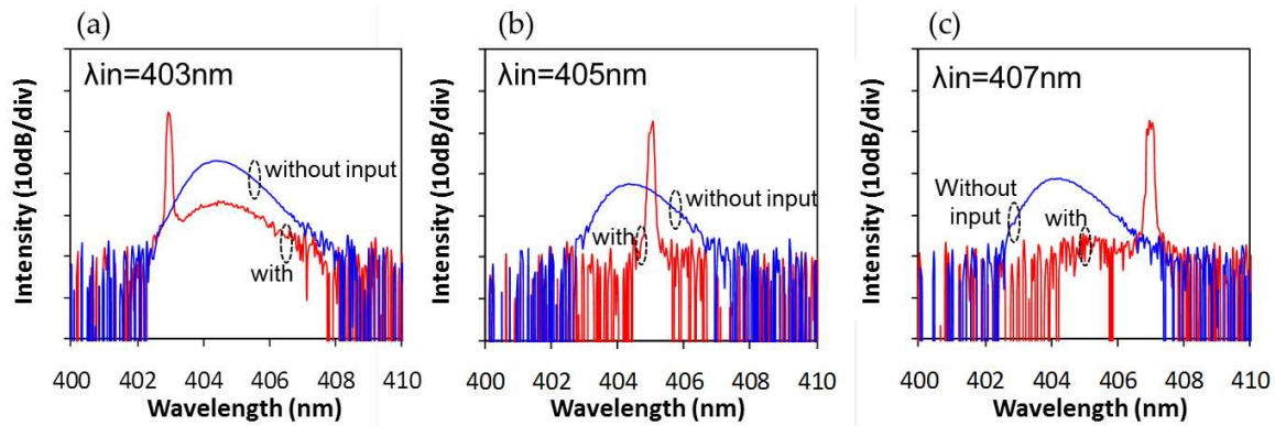
Figure 7. Optical spectra of the output of an angled SOA obtained with input wavelengths of (a) 403, (b) 405, and (c) 407 nm. Current density and input power were 4 \text{ kA/cm}^2 and 11 \text{ mW} , respectively. Spectra with (red) and without (blue) input are shown for each wavelength.
