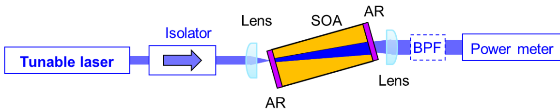
Figure 5. Experimental setup for CW amplification.
