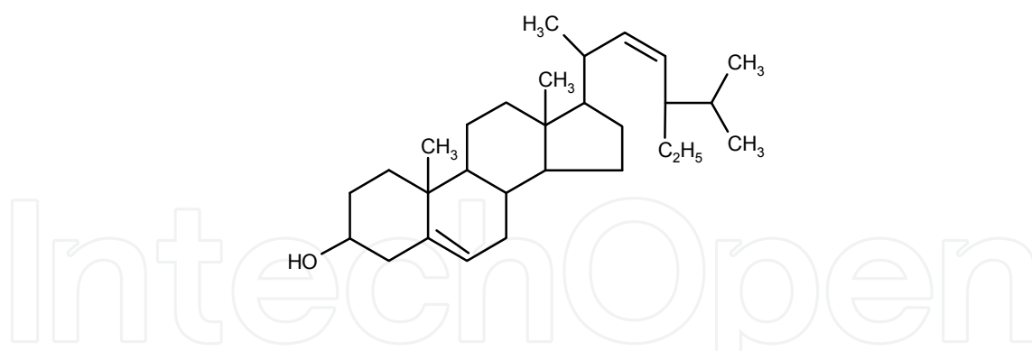
Figure 9. Fucosterol, also known as [24 (28) E]-estigmasta-5, 24 (28)-diene-3 \beta -ol, [24 (24') E] -estigmasta-5, 24 (24') -di-en-3 \beta -ol or 24E-etilidenecolesta-5, 24 (28) -diene-3 \beta -ol. Chemical formula C 29 H 48 O, PM 412.69. [52, 53]
