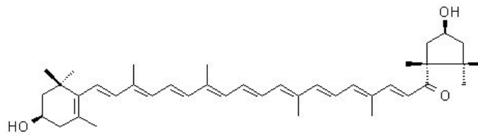
Capsanthin: Present in peppers, paprika
