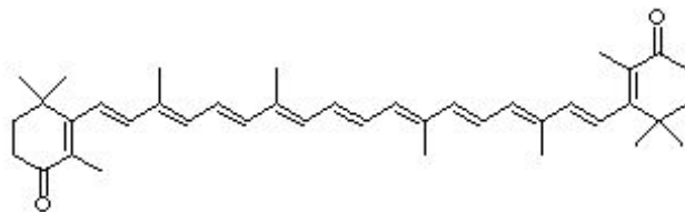
α-carotene: Present in: carrots, most green plants
