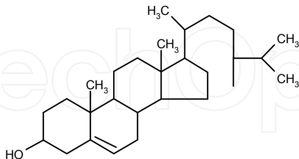
Figure 6. Campesterol or 24 \alpha -methyl-5-cholesten-3 \beta -ol, 24 \alpha -metilcolesterol, 24(R)-metilcolesterol, (24R)-5-ergosten-3- \beta -ol. Chemical formula C 28 H 48 O, MW 400.68 and melting point of 157–158°C. [52, 53]
