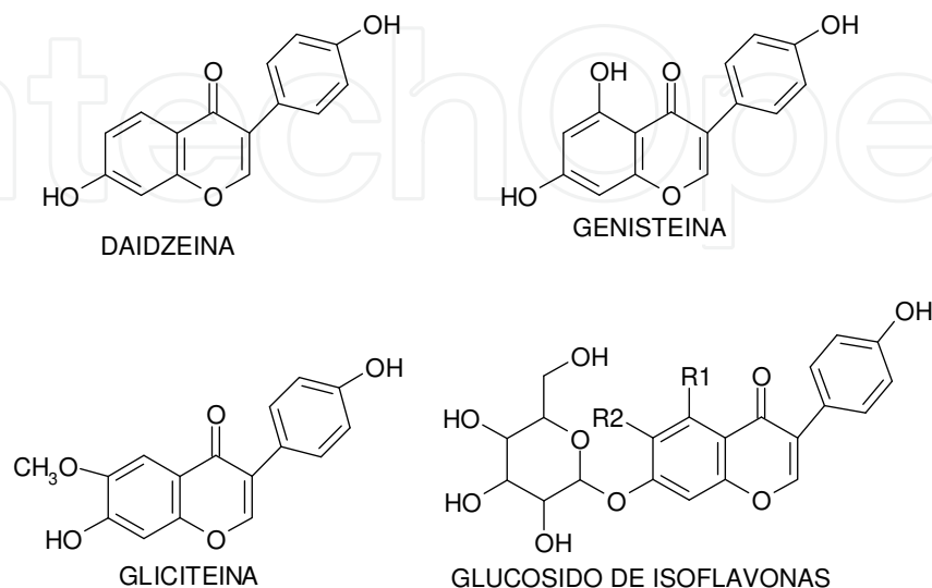
Figure 5. Isoflavones structure
