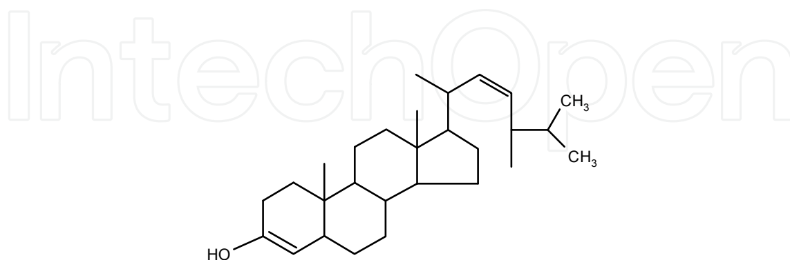
Figure 10. 5-avenasterol (5-avenasterol), called isofucosterol, 28-isofucosterol, 29-isofucosterol, 24Z-etilidenecolesta-5, 24 (28) -diene-3 \beta -ol, [24(28Z)] -estigmasta-5, 24 (28) -diene-3 \beta -ol or [24(24')-Z]-estigmasta-5, 24(28')-diene-3 \beta -ol, chemical formula C 29 H 48 O, PM 412.69. [52, 53]
