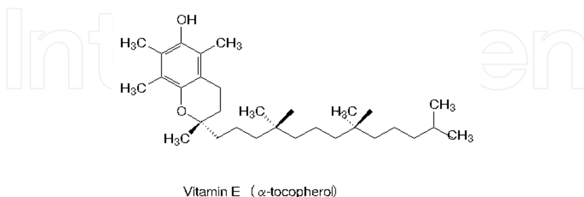
Figure 2. Vitamin E structure
