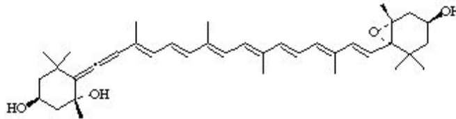
Neoxanthin: Present in the chloroplasts of most plants
