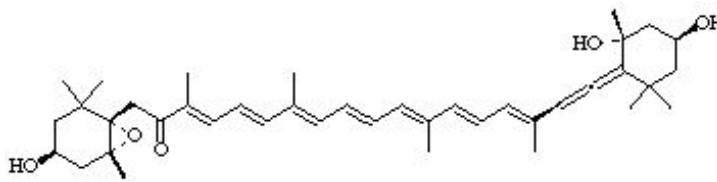
Fucoxanthinol: Present in many algae and seaweed
