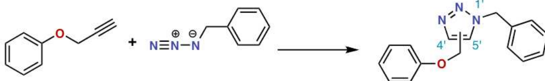
Figure 4. Azide–alkyne Huisgen cycloaddition “click” reaction
