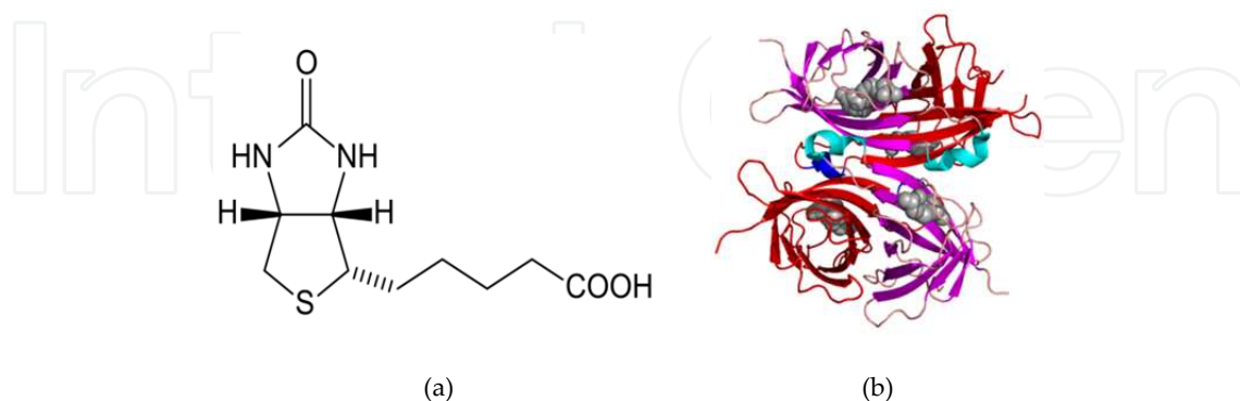
Figure 5. Biotin structure (a) and the simple graph for biotin–avidine binding (b)
