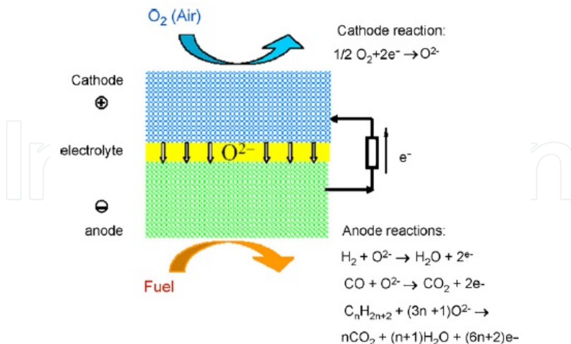
Figure 8. Schematic diagram showing the working principle of a solid oxide fuel cell [157].
