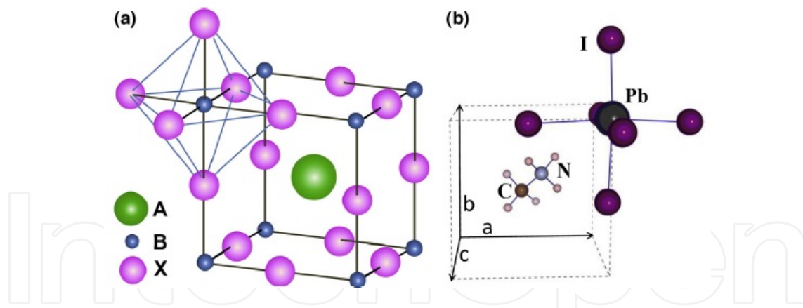
Figure 9. (a) \text{ABX}_3 perovskite structure showing \text{BX}_6 octahedral and larger A cation occupied in cubo-octahedral site. (b) Unit cell of cubic \text{CH}_3\text{NH}_3\text{PbI}_3 perovskite [171].
