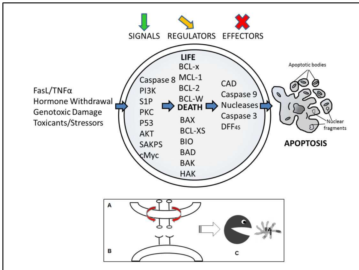
Figure 1. Top: signals, regulators and effectors involved in the balance between life and death. Left, the main inductors of apoptosis. Bottom, exemplification of the exposure mechanism of PS from the inner to the outer membrane of an apoptotic cell. (A) PS exposure in the apoptotic cell and (B) PS receptors of the phagocyte. (C) This specific recruitment consents the engulfment of the apoptotic cell or apoptotic bodies and their clearance.
