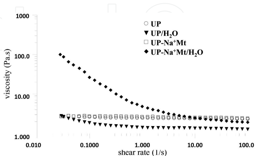
Figure 8. Shear viscosity for the systems UP, UP/H 2 O, UP-Na + Mt 5 phr clay, and UP-Na + Mt/H 2 O 5 phr clay.
