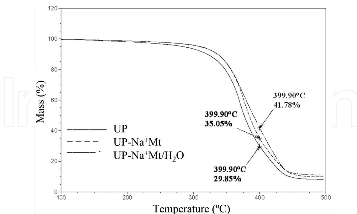
Figure 6. Mass loss from TGA analysis for UP, UP-Na + Mt/H 2 O 5 phr clay, and UP-Na + Mt 5 phr clay.
