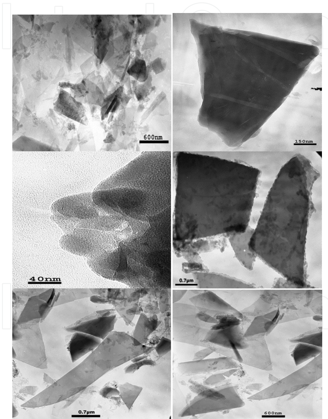
Figure 2. TEM micrographs of metanacrite synthetic material [29].
