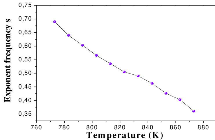
Figure 4. Temperature dependence of frequency exponent( s ) for metanacrite sample [29].
