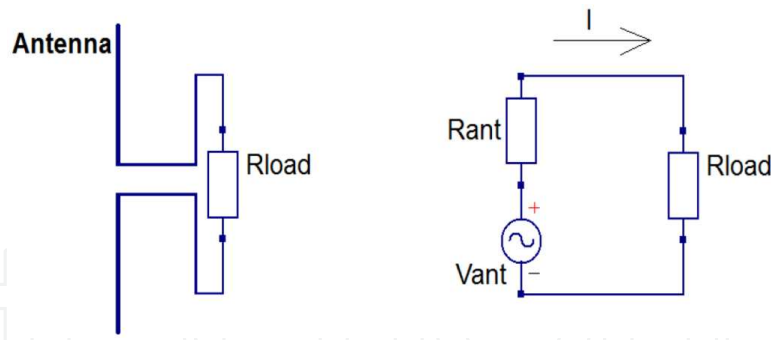
Figure 1. Antenna equivalent circuit.
