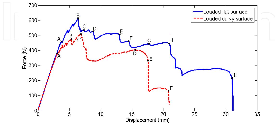
Figure 9. Comparison between the bending responses of two woven composite specimens with different loaded surfaces. For flat surface loaded sample : Point A: Initiation of fiber micro buckling in the first (top) layer, Point B: Completion of failure in the first layer, Point F: complete compression failure in the second layer, Point C and G: Delamination occurrence, Point H: Onset of fiber tensile failure in the lowest layer ( 6^{\text{th}} ), Point I: Complete fiber breakage in 5^{\text{th}} layer. For curvy surface loaded sample : Point A: Initiation of fiber micro buckling in the first (top) layer, Point B: Completion of failure in the first layer, Point C: Complete compression failure in the second layer, Point D: Nucleation of fiber breakage in the lowest layer, Point E: Complete failure in the lowest layer, Point F: Complete fiber tensile failure in the 5^{\text{th}} layer [68].
