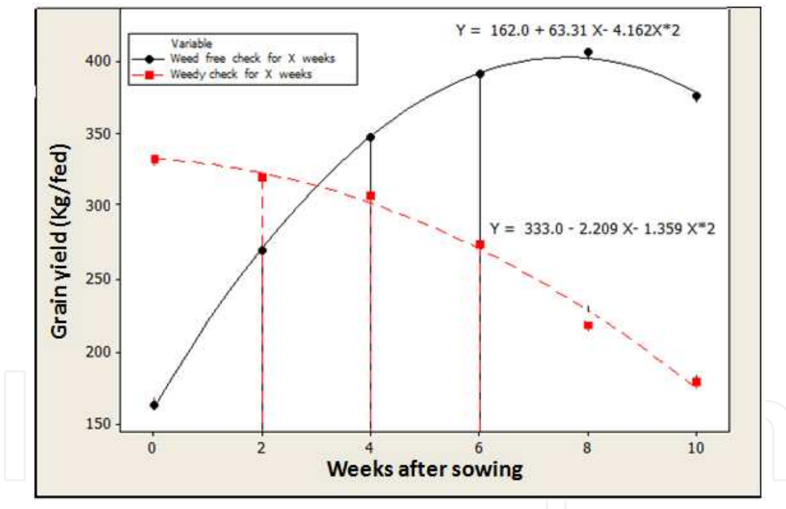
Figure 2. Critical period of weed interference in sesame.
