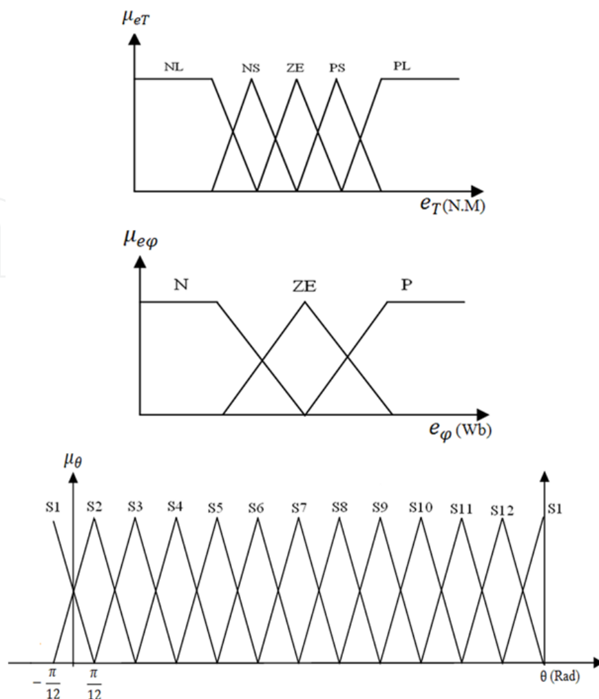
Figure 3. Membership functions.
