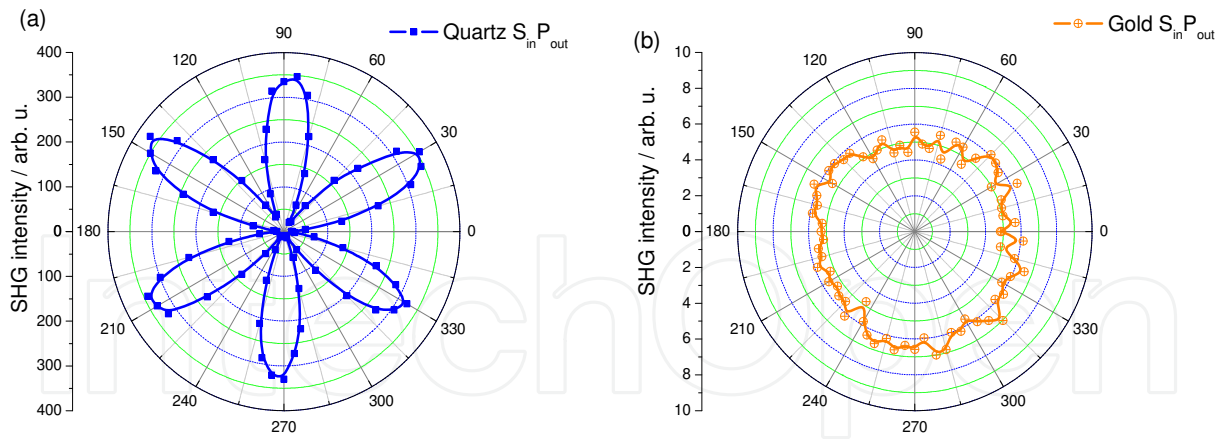
Figure 10. SHG measurements as a function of sample orientation ( \Omega ) for (a) z-cut \alpha -quartz and (b) thermally evaporated gold film, with the S_{in}P_{out} polarization combination.
