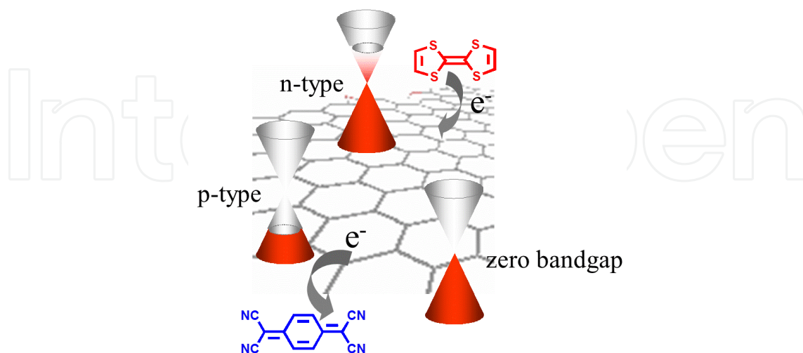
Figure 3. Doping graphene with semiconductor donor and acceptor molecules move the Fermi level up or down with respect to the Dirac point.
