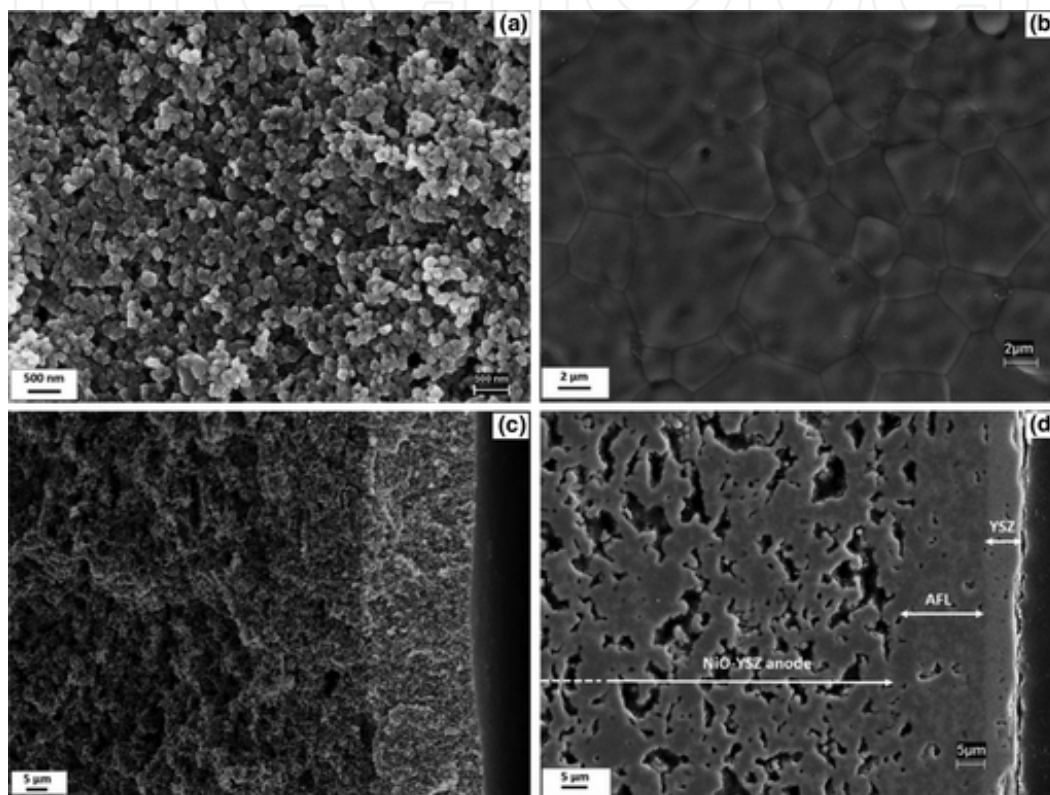
Figure 3. Field-emission SEM images of top view and cross-section of yttria-stabilized zirconia (YSZ) electrochromic deposition coating (a) (c) as-deposited and (b) (d) sintered at 1400 °C for 6 h, directly deposited onto the conducting polymers such as polypyrrole-coated NiO-YSZ substrate at a constant applied voltage of 15 V. Reprinted from [31], with permission from John Wiley and Sons.
