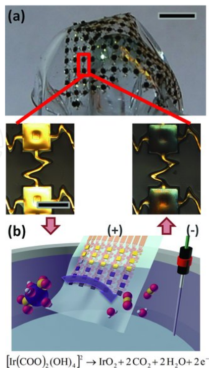
Figure 5. (a) Picture of the produced pH sensors with the magnified images of the gold electrodes before (lower left) and after (lower right) \text{IrO}_x electroplating. The scale bars correspond to 5 and 0.5 mm for the upper and the lower images, respectively. (b) Schematic illustration of the chemical reactions during \text{IrO}_x electroplating. Reprinted from [38], with permission from John Wiley and Sons.
