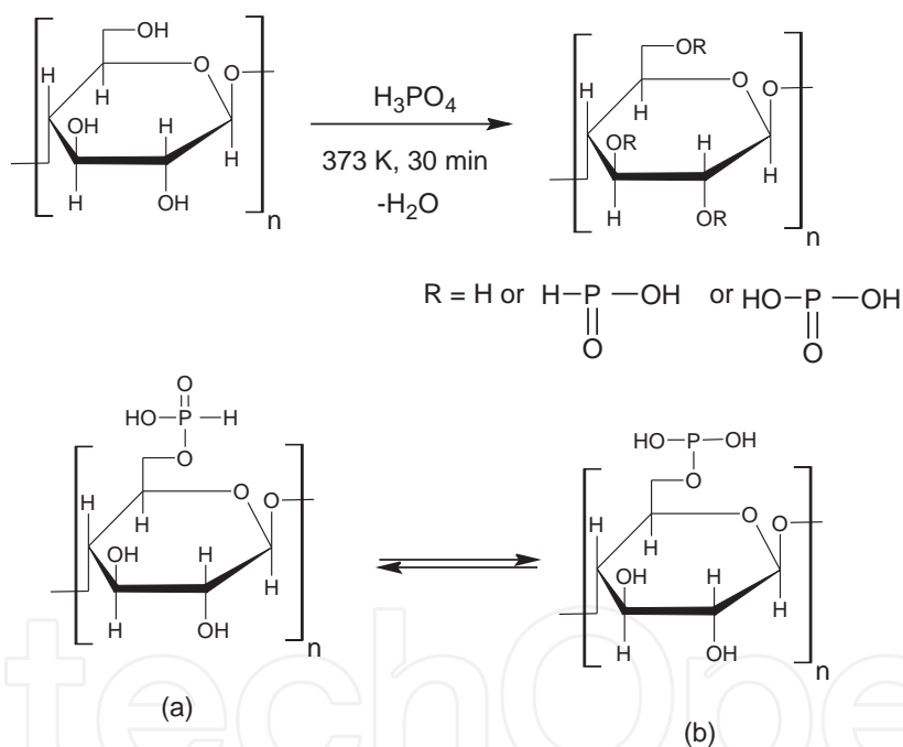
Figure 4. Reaction scheme of cellulose phosphorylation with H_3PO_4 in aqueous medium, and possible tautomeric products (a and b) of phosphated cellulose structure.
