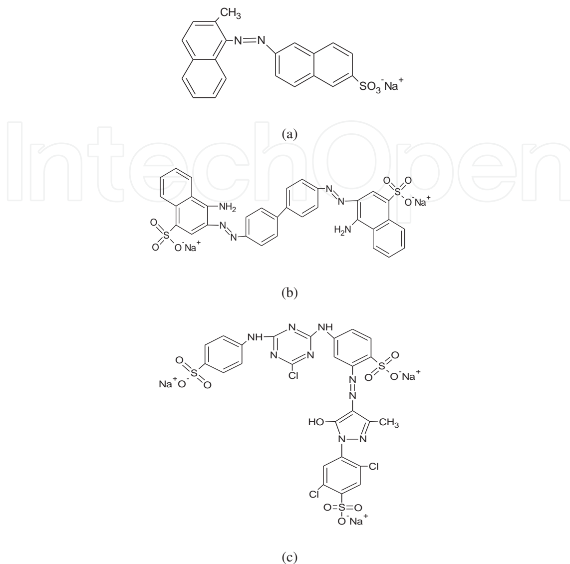
Figure 16. Chemical structure of the red acid dyes GR (a), congo red 4BS (b), and pale yellow reactive K-4G (c).
