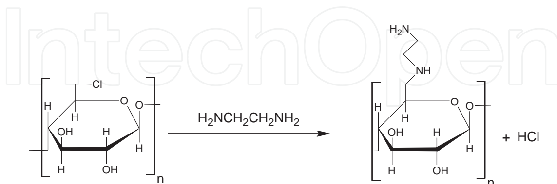
Figure 12. Reaction of chlorinated cellulose with ethylene-1,2-diamine.
