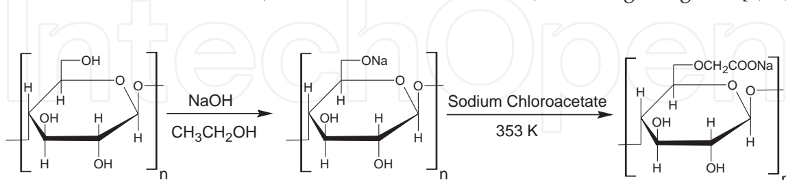
Figure 2. Preparation scheme of the CMC.
