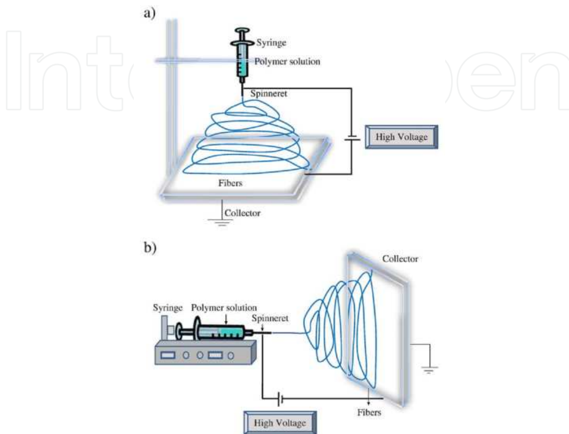
Figure 4. Schematic representation illustrating the set up of an electrospinning apparatus. A) typical vertical set up, b) horizontal setup. Reprinted with permission from ref [59]. Copyright 2010 Elsevier.
