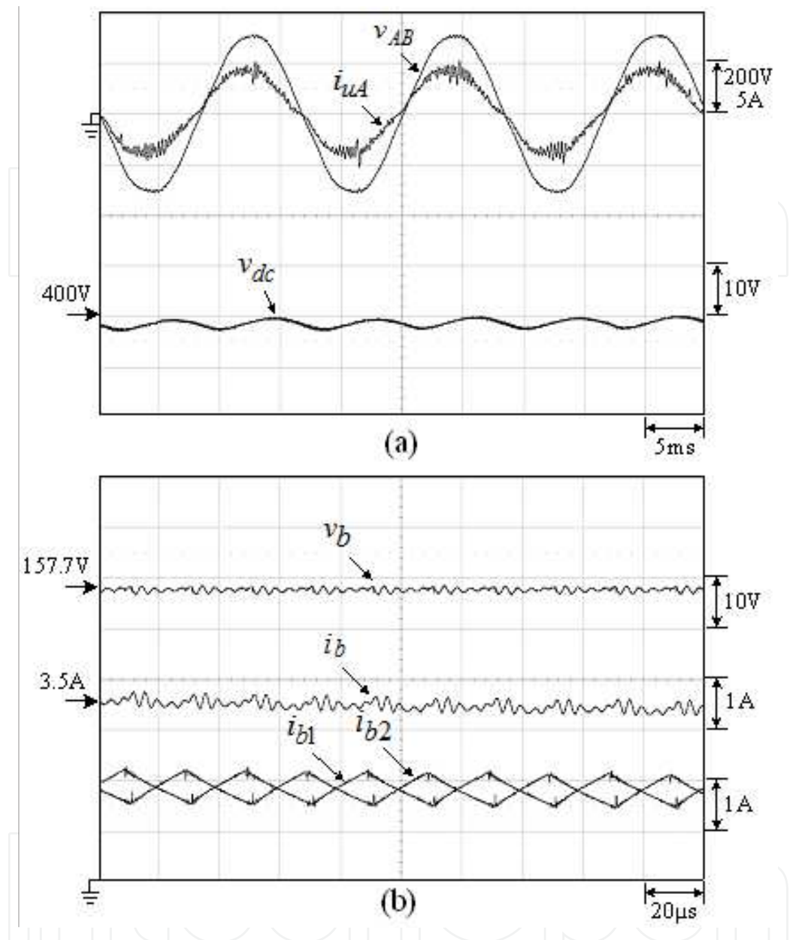
Figure 18. Measured results of the established single-phase charging system at ( i_b^* = 3.5\text{A} , V_b = 157.7\text{V} , V_{dc}^* = 400\text{V} , V_{AB} = 220\text{V}/60\text{Hz} ): (a) ( v_{dc} , v_{AB} , i_{uA} ); (b) ( v_b , i_b , i_{b1} , i_{b2} ).
