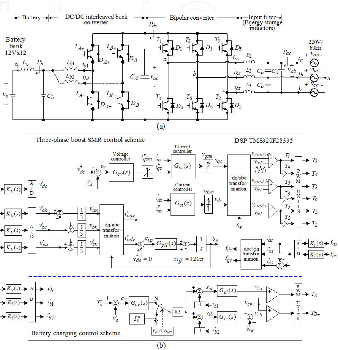
Figure 19. Schematic and control scheme of the established three-phase SMR based battery charger: (a) schematic; (b) control scheme.
