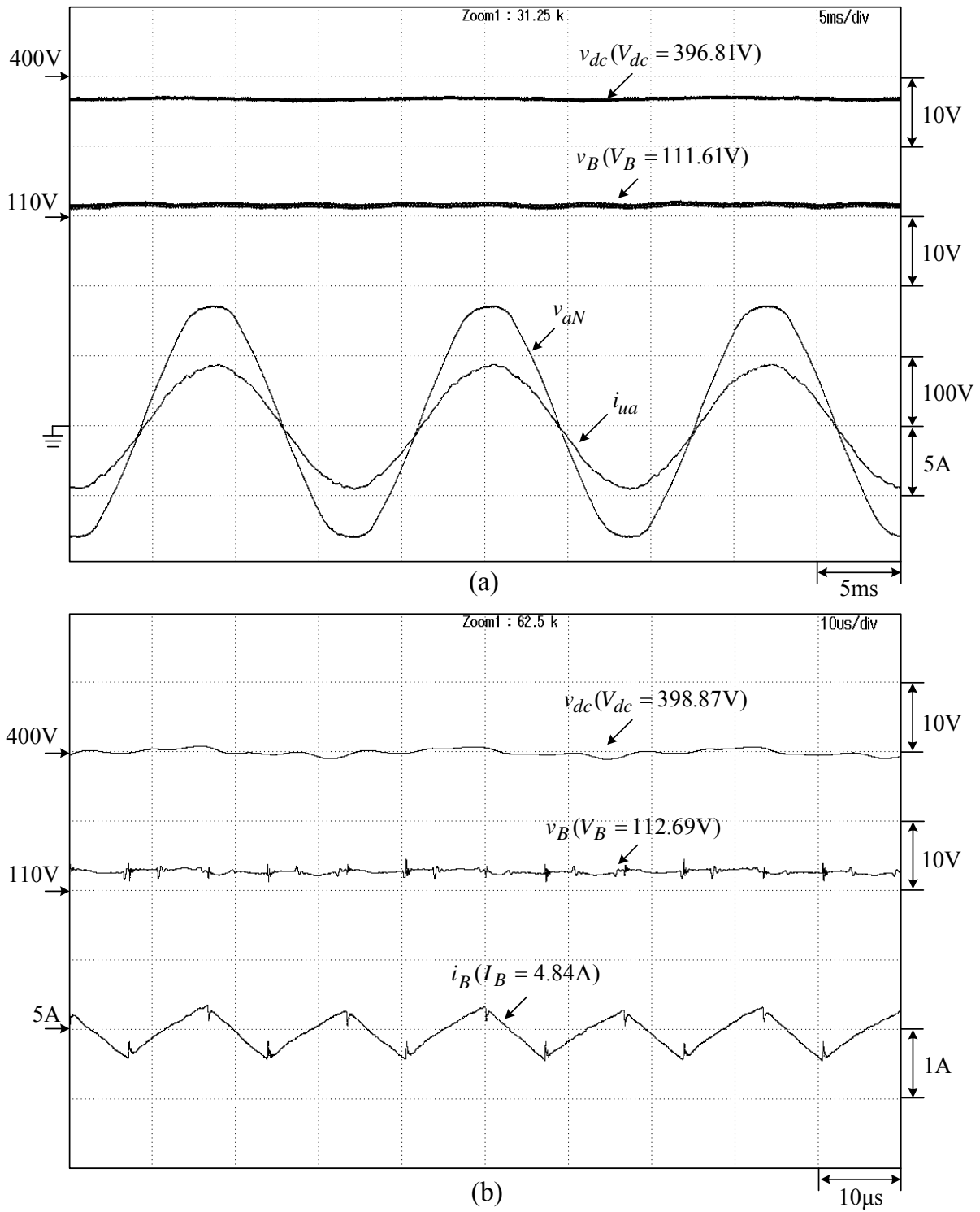
Figure 13. Measured results of the established BESS in charging modes at linear resistive and induction motor reactive load: (a) v_{dc} , v_B and (v_{aN}, i_{ua}) ; (b) v_{dc} , v_B and i_B .
