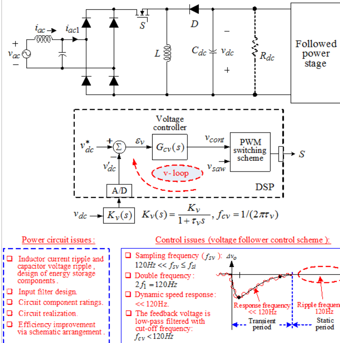
Figure 6. Some key issues of single-phase buck/boost SMRs.
