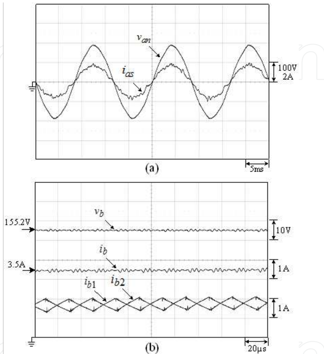
Figure 20. Measured ( v_{an} , i_{as} ) and ( v_b , i_b ) of the established three-phase SMR based battery charger at ( i_{bm}^* = 0.25C = 3.5A , V_{ab} = 220V/60Hz , V_{dc} = 400V , V_b = 155.2V ): (a) ( v_{an} , i_{as} ); (b) ( v_b , i_b , i_{b1} , i_{b2} ).
