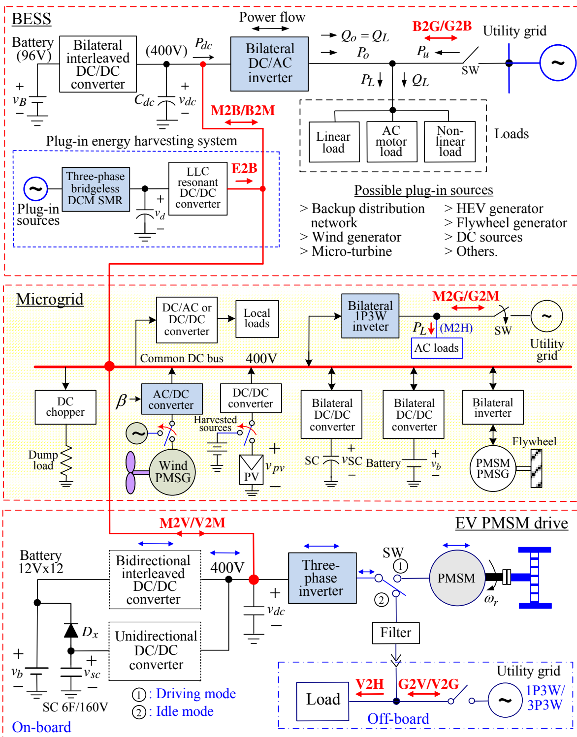
G2V: grid-to-vehicle, V2G: vehicle-to-grid, V2H: vehicle-to-home, M2G: microgrid-to-grid, M2V: microgrid-to-vehicle, V2M: vehicle-to-microgrid, E2B: energy-harvester-to-BESS, B2G: BESS-to-grid, G2B: grid-to-BESS, M2B: microgrid-to-BESS, B2M: BESS-to-microgrid.
