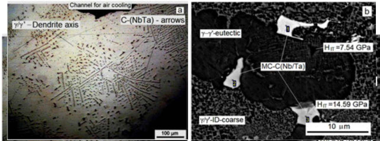
Figure 12. Interdentritic region in turbine blade cross-section with air cooling channel (top) and MC-(Nb/Ta) metal carbide (bottom) for reinforcement of the interdentritic region (a) and MC near the eutectic pool in the interdentritic region (b).
