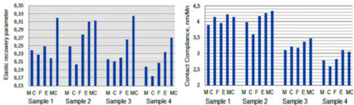
Figure 24. The phase dependence of the elastic recovery (a) and contact compliance (b) parameters for samples under cumulative strain. Designations such as those in Figure 22 are shown.
