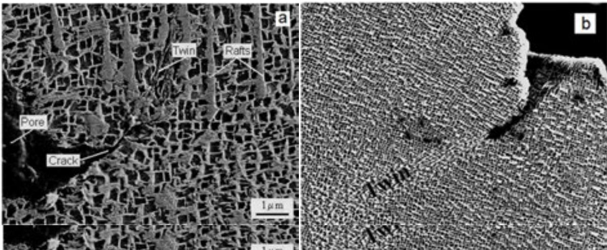
Figure 34. Rafts and twins forming during HCV deformation (a) and deformation twinning and its related fracture during TMF cycling of four nickel-based single-crystal superalloys (b). Adapted from references [28, 51].
