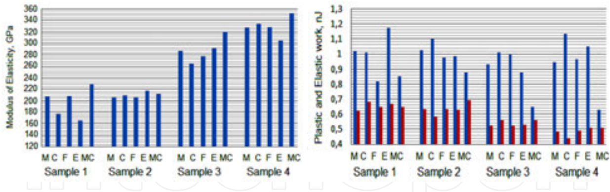
Figure 23. The phase dependence of the elastic modulus (a) and both the plastic and elastic work (b) for samples from collected strains. Designations such as those in Figure 22 are shown.
