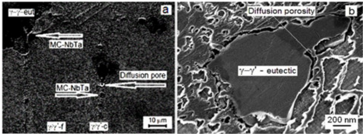
Figure 30. Diffusion micropore (a) and phase/grain boundaries (b) forming in SC as a result of the absence of balanced interdiffusion during HCV deformation.
