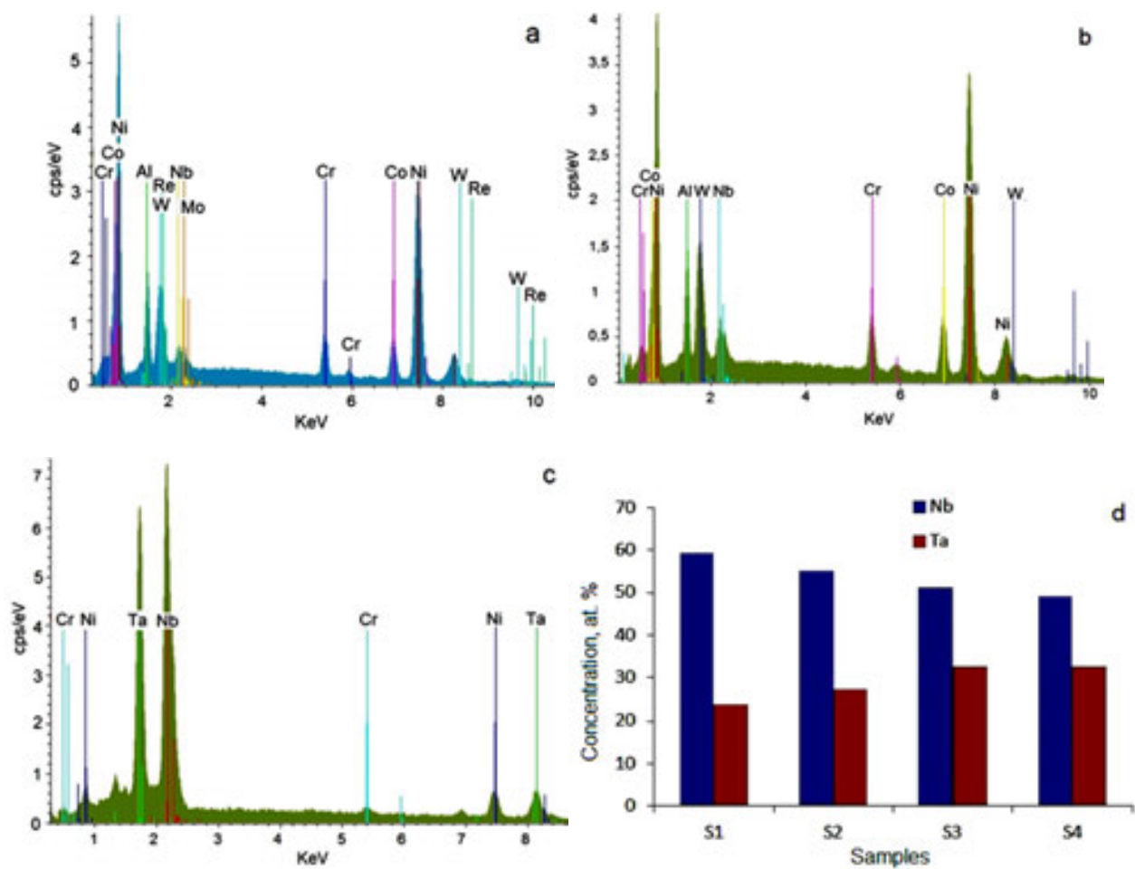
Figure 31. SEM-EDS diagrams of the sample (S4) in the primary dendrite axis or fine \gamma/\gamma' -phase (a), in the eutectic \gamma-\gamma' phase region (b), in the MC phase (c), and Nb/Ta content evolution at interdiffusion in the MC phase (d) of samples.
