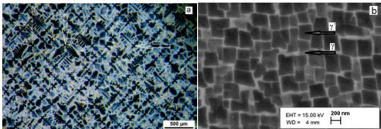
Figure 10. Microstructure of as-cast SC Ni-based superalloy ZS32-vi in cross-section of rod (a) and \gamma/\gamma' phase (b). The primary dendrite quadrature axis and \gamma and \gamma' phases are shown by arrows.
