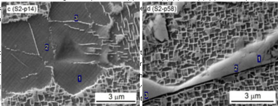
Figure 22. Nanoindentation triangular test points in the \gamma/\gamma' -coarse (a), \gamma/\gamma' -fine (b), \gamma-\gamma' -eutectic pool (c), and C(Nb/Ta)-MC (d) phases. The chemical elemental compositions of the three measured points by SEM EDS in these phases are shown near the indents. Adapted from reference [46].
