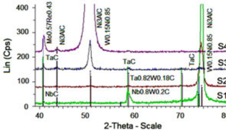
Figure 32. X-ray diffraction diagrams of samples S1, S2, S3, and S4 for different cumulative strains. Adapted from reference [43].
