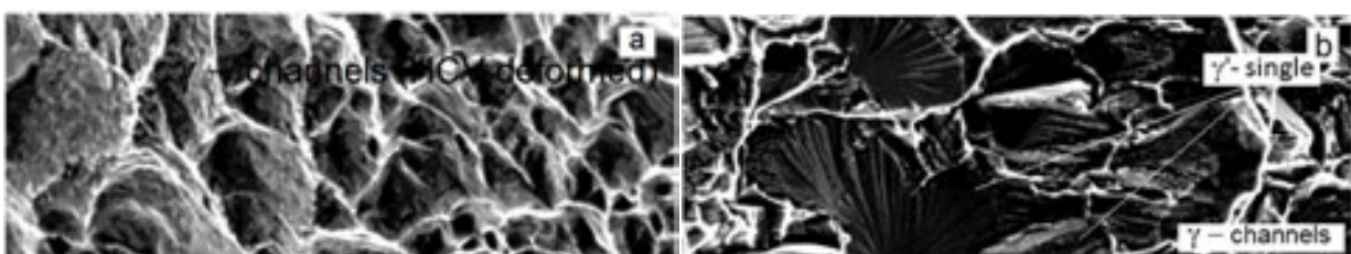
Figure 35. PDA in cross-section (a) and fracture of a preliminarily HCV deformed SC by PDA in (001) direction. Adapted from reference [28].
