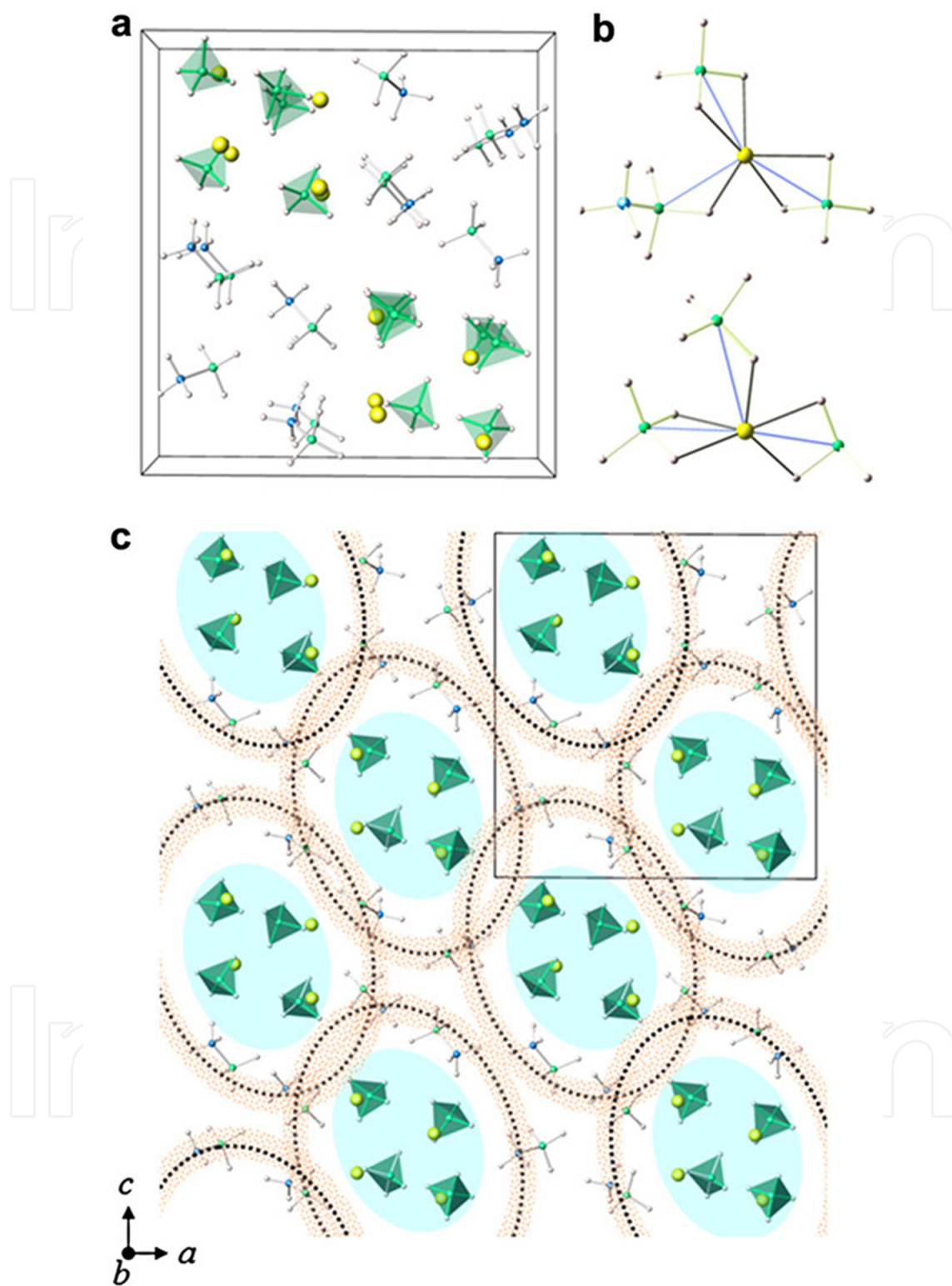
Figure 25. (a) Crystal structure of \text{LiBH}_4 \cdot \text{AB} . (b) \text{Li}^+ coordination. (c) Schematic arrangement of \text{LiBH}_4 and \text{AB} components in the crystal structure. Li: yellow spheres; B: green spheres; N: blue spheres; and H: white spheres. Reproduced from Ref. [77] with permission.
