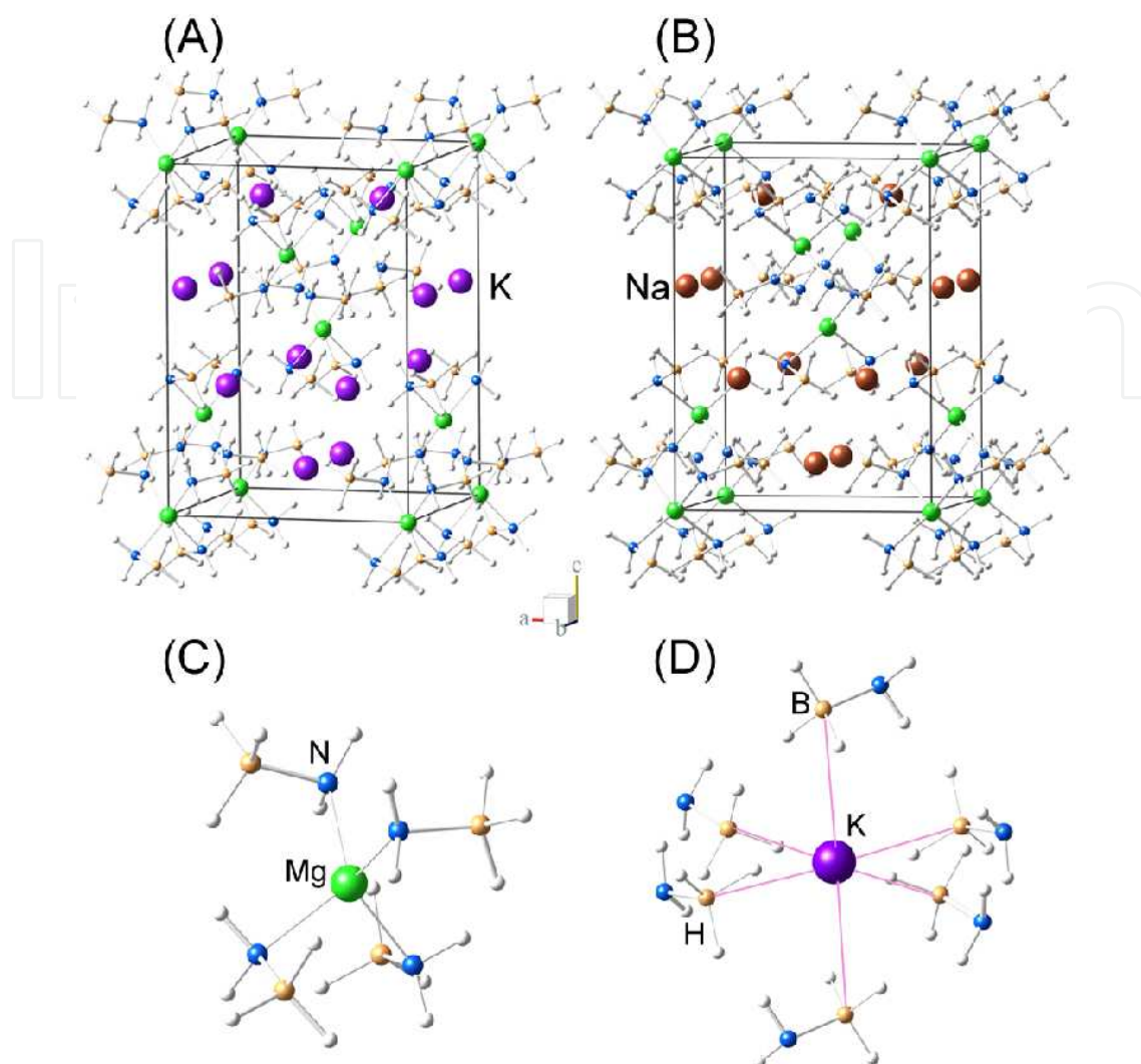
Figure 20. Crystal structure of (a) K_2Mg(NH_2BH_3)_4 , (b) Na_2Mg(NH_2BH_3)_4 , (c) Coordination of Mg^{2+} , and (d) Coordination of K^+ . Reproduced from Ref. [62] with permission.
