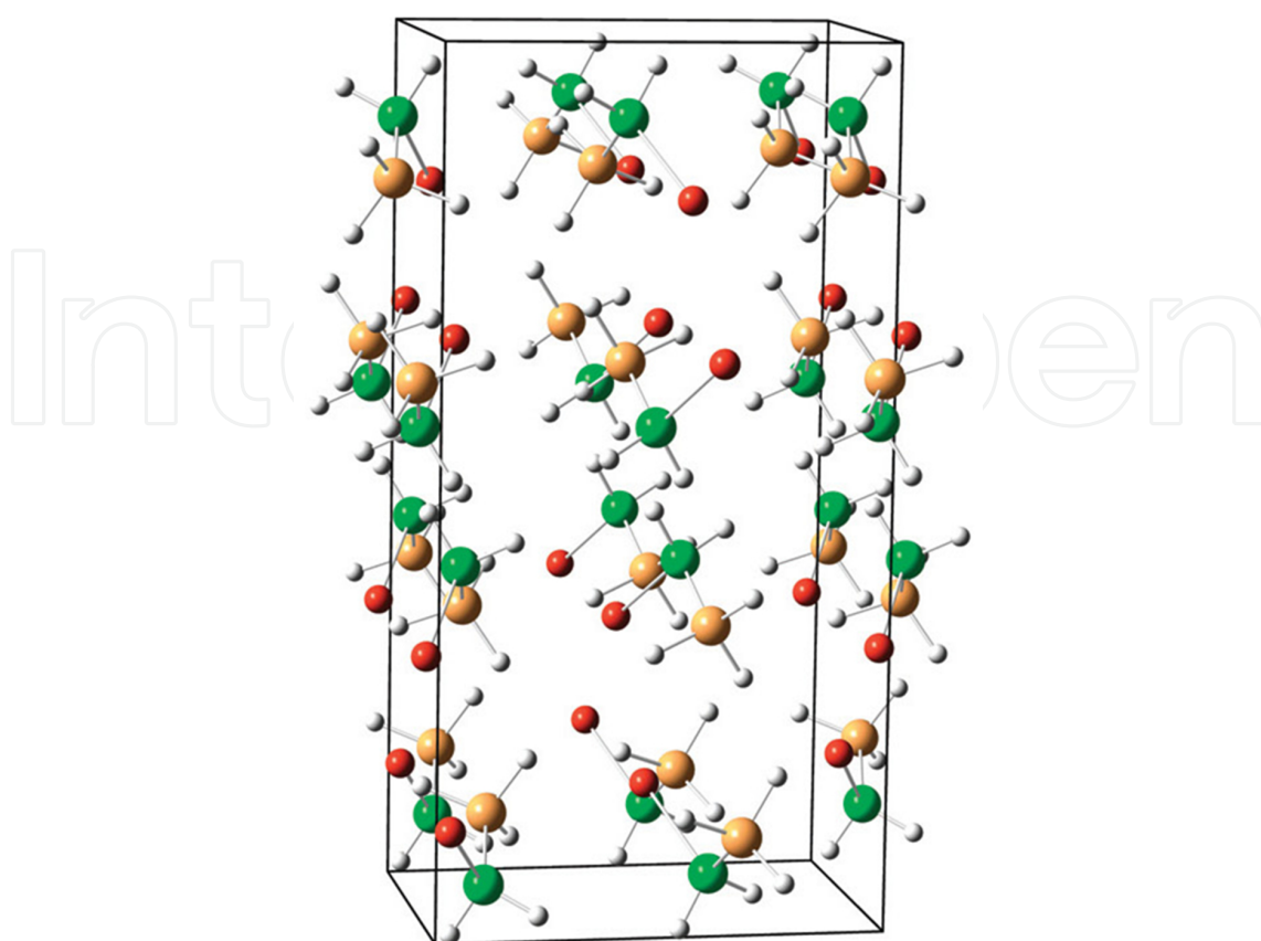
Figure 11. Crystal structure of LiAB. B: orange spheres; N: green spheres; H: white spheres; and Li: red spheres. Reproduced from Ref. [36] with permission.
