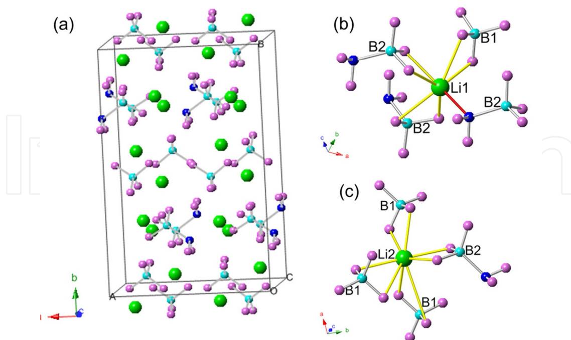
Figure 28. (a) Crystal structure of \text{LiAB} \cdot \text{LiBH}_4 and (b, c) Coordination of \text{Li}^+ . Li: green spheres; N: blue spheres; B: cyan spheres; and H: pink spheres. Reproduced from Ref. [85] with permission.
