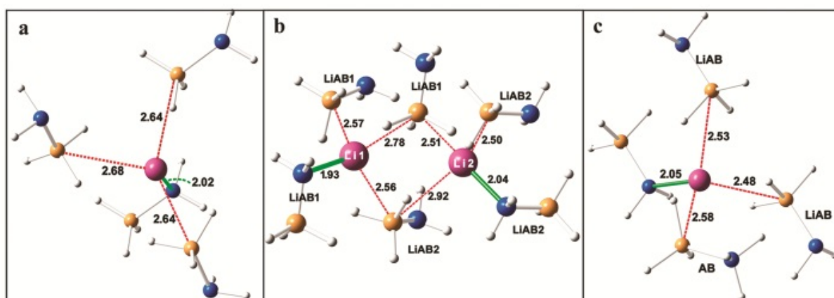
Figure 13. Coordination of Li + in (a) \alpha -LiAB, (b) \beta -LiAB, and (c) LiAB·AB. Li: purple spheres; B: brown spheres; N: blue spheres; and H: white spheres. Reproduced from Ref. [53] with permission.
