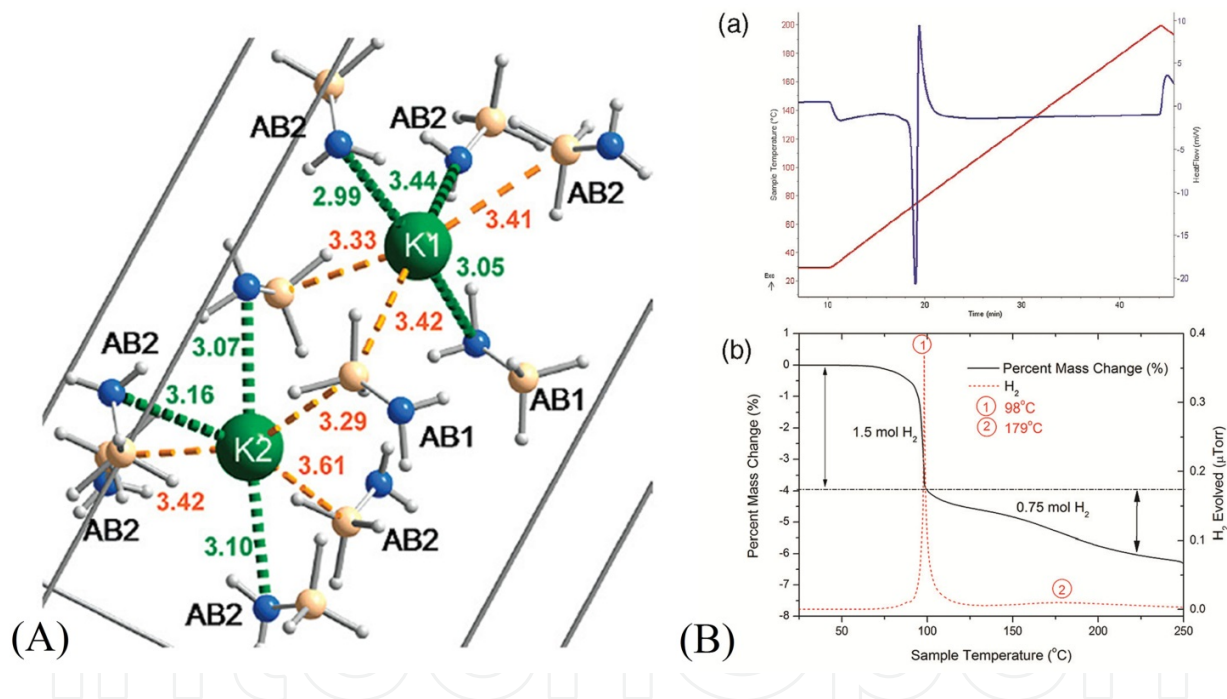
Figure 14. (A) Crystal structure of KAB. K: green spheres; N: blue spheres; B: cream spheres; and H: white spheres. (B) (a) DSC and (b) IGA data for KAB decomposition. Reproduced from Ref. [40] with permission.
