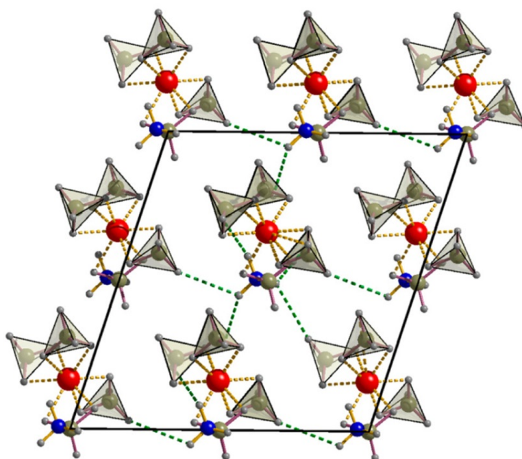
Figure 27. Crystal structure of \text{Al}(\text{BH}_4)_3 \cdot \text{AB} : (a) \alpha -phase and (b) \beta -phase. Reproduced from Ref. [80] with permission.
