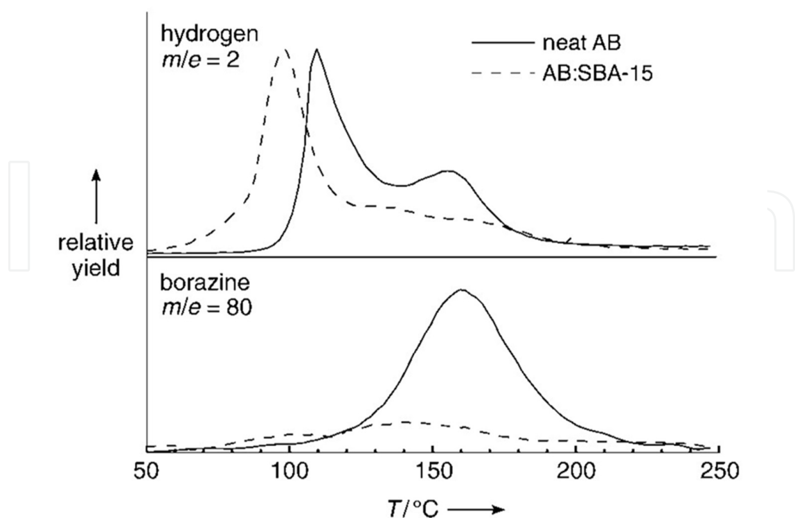
Figure 1. TPD/MS tests of AB nanoconfined in SBA-15 (AB:SBA-15). For comparison, neat AB was also included. Reproduced from Ref. [6] with permission.
