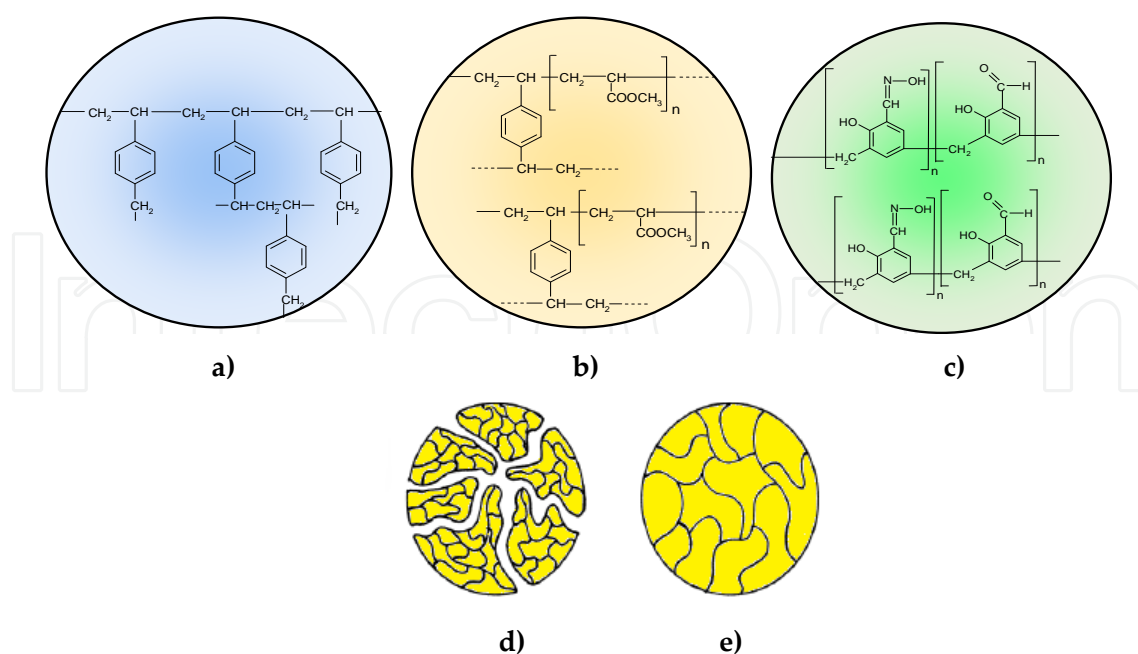
Figure 4. Composition of resin matrices: a) styrene-divinylbenzene skeleton, b) acrylic-divinylbenzene skeleton, c) phenol-formaldehyde skeleton, and their structure: d) macroporous, e) gel
