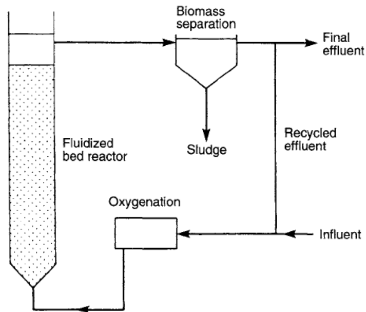
Figure 22. Typical design of fluidized bed reactor system [1].
