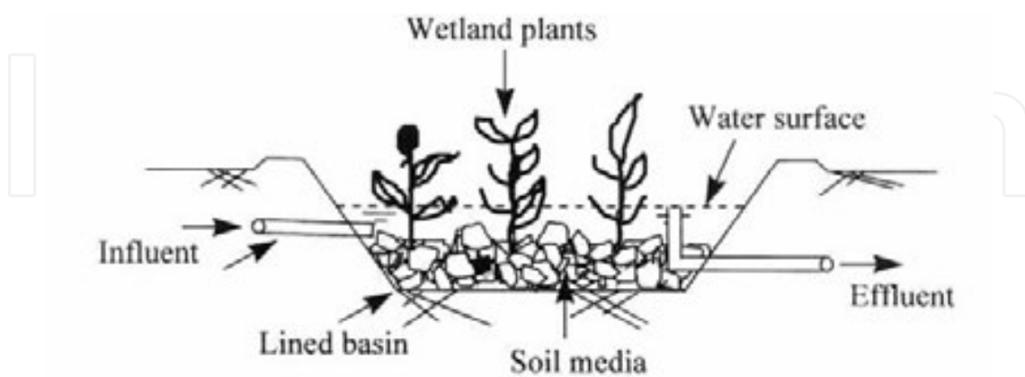
Figure 41. Free water surface system [18].
