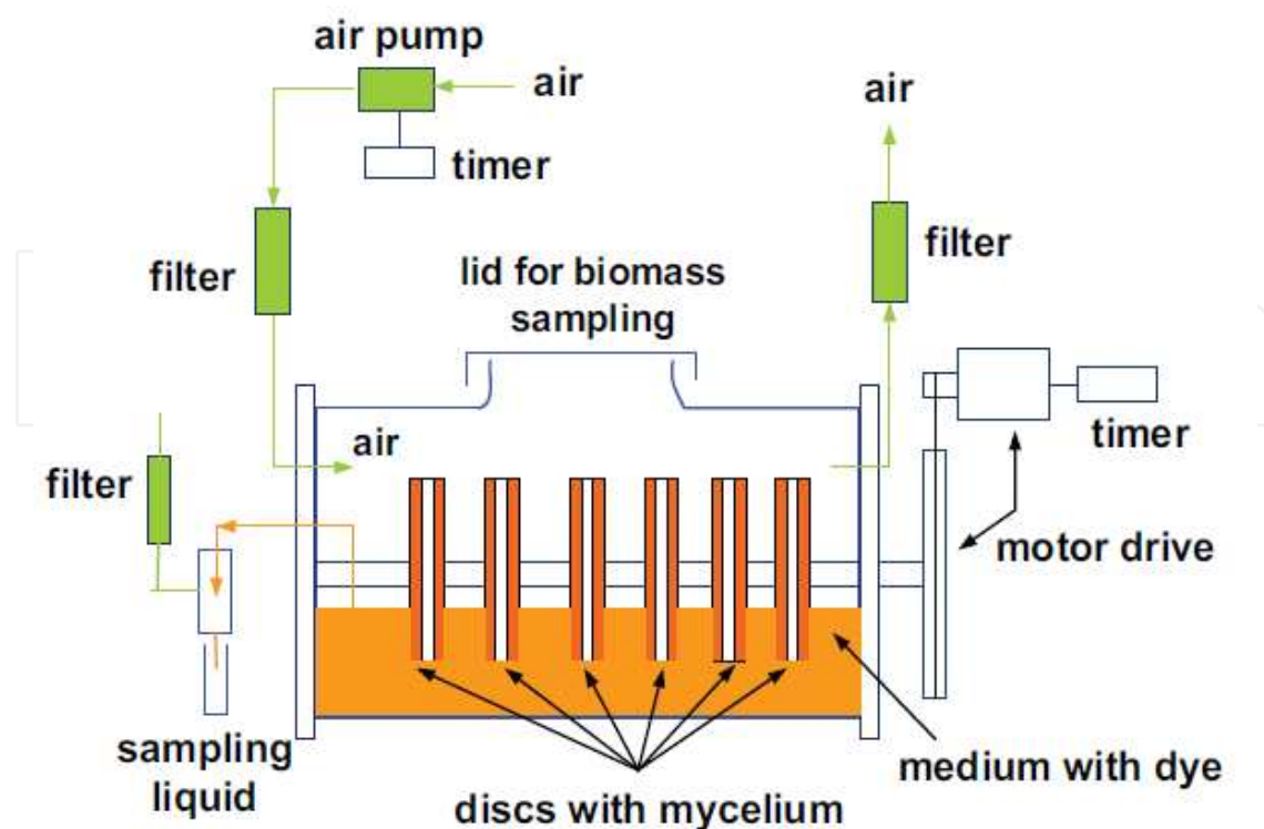
Figure 20. A bioreactor for fungal degradation: rotating disc bioreactor [13].
