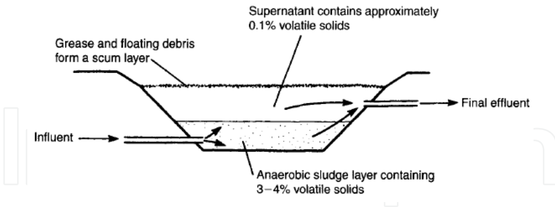
Figure 16. Anaerobic lagoon for strong wastewater treatment, such as meat processing wastewater [1].
