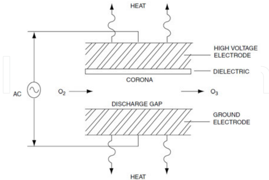
Figure 52. Schematic drawing of corona discharge method for making ozone [3].
