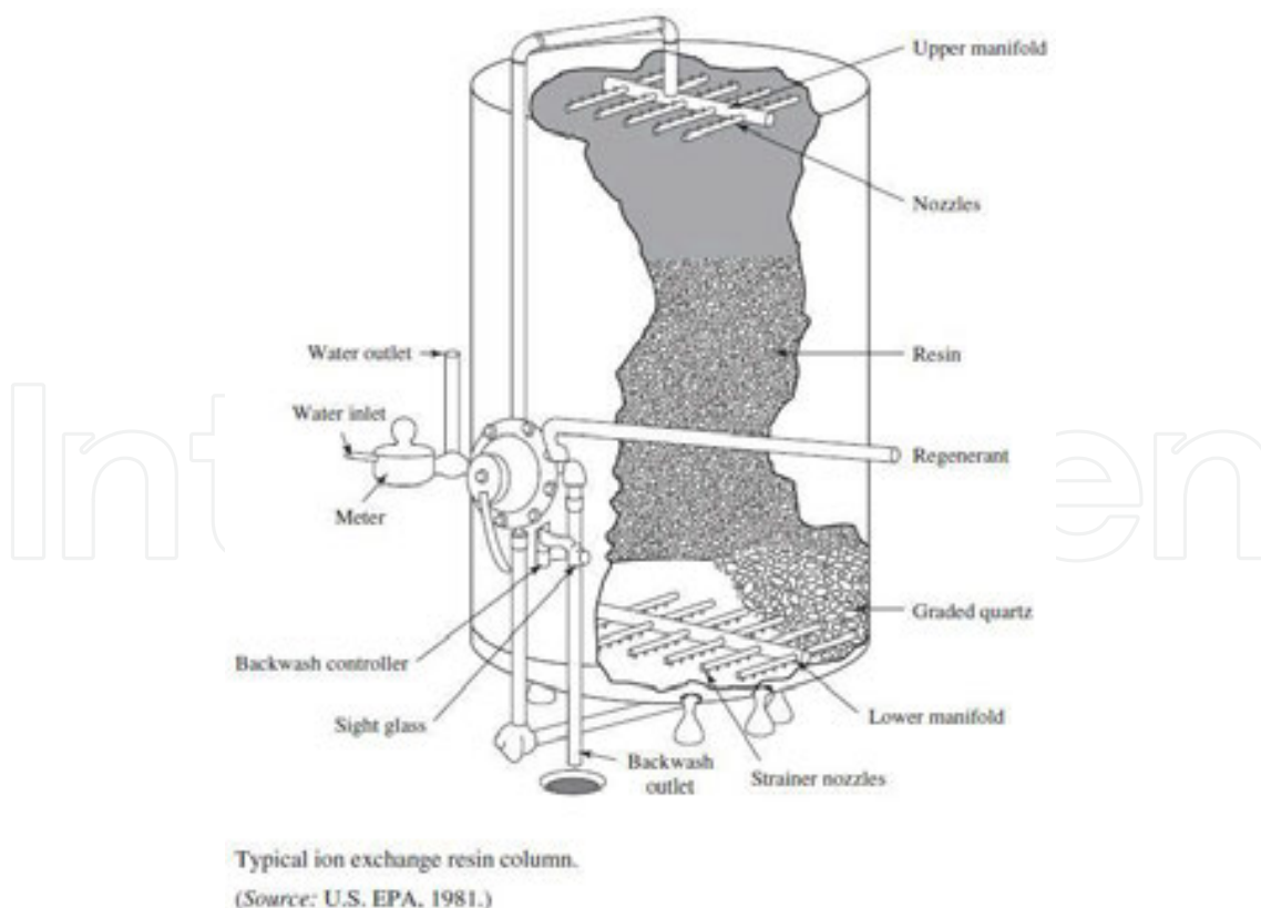
Figure 54. Typical ion exchange resin column [37].
