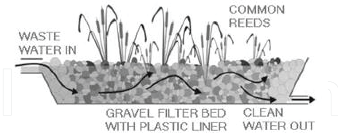
Figure 39. Cross-sectional view of a typical subsurface flow constructed wetland [17].
