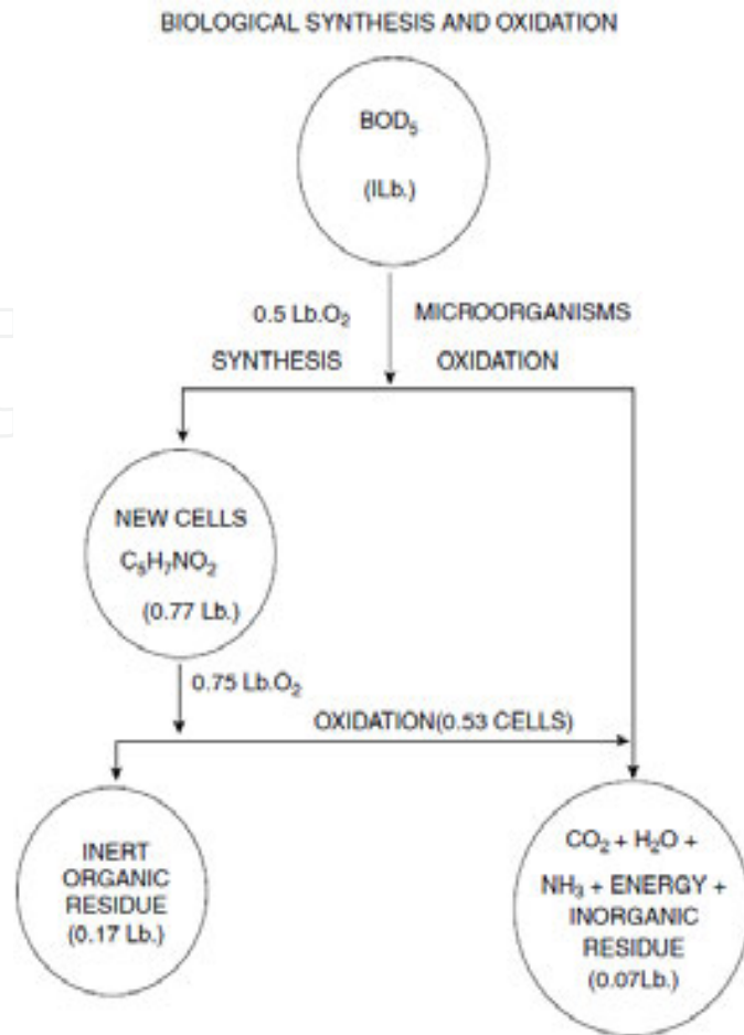
Figure 1. Biological synthesis and oxidation [3].
