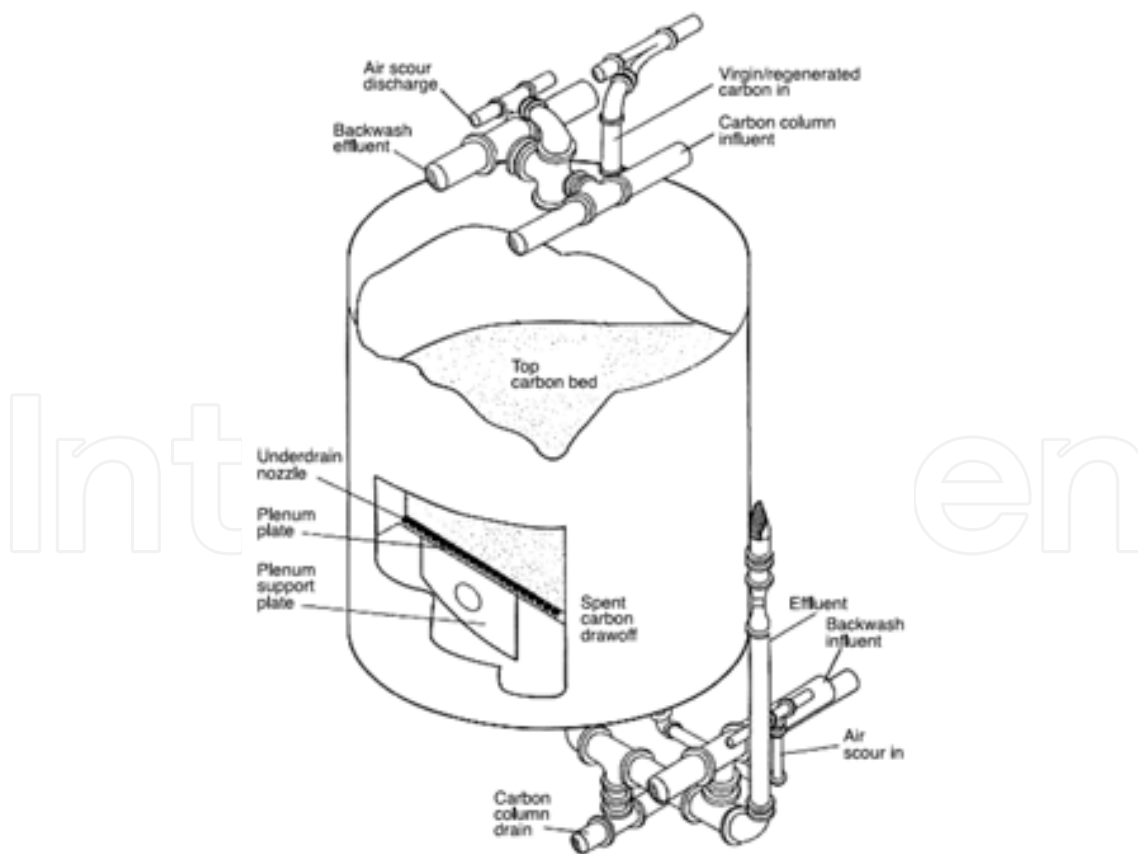
Figure 50. A bed carbon adsorption unit [35].
