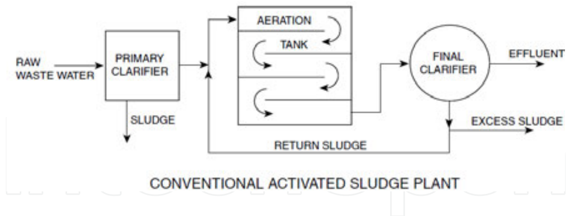
Figure 24. Conventional activated sludge plant [3].
