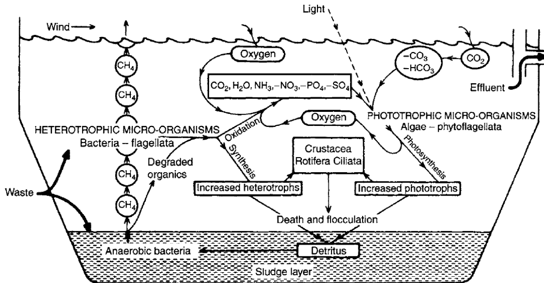
Figure 5. Aerobic system/oxidation pond [1].
