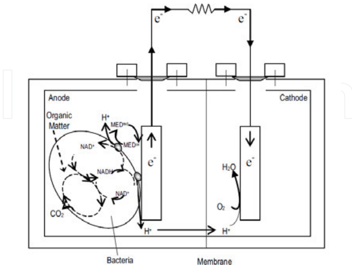
Figure 48. Schematic diagram of the essential components of an MFC [33].
