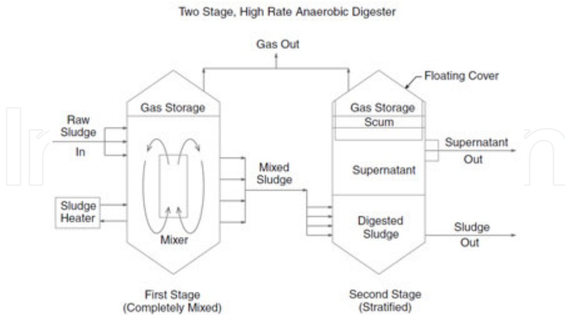
Figure 10. Dual-stage high rate digester [3].
