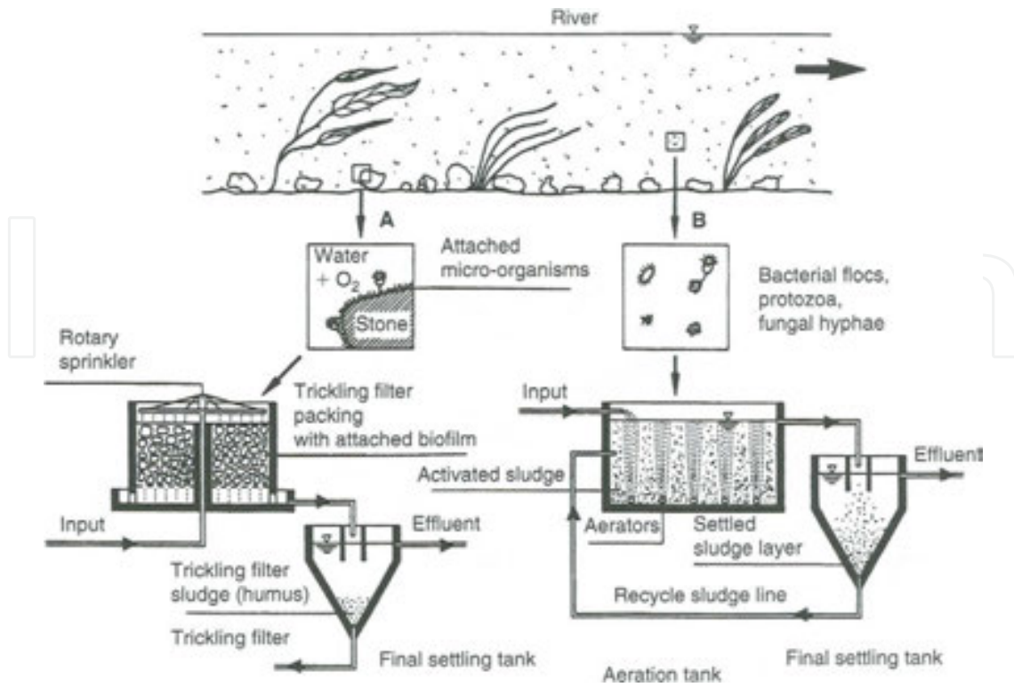
Figure 31. Relationship between the natural bacterial populations in rivers and the development of (A) trickling (percolating) filter and (B) activated sludge system [1].
