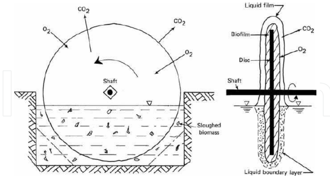
Figure 34. Mechanism of attached growth media in an RBC system [2].
