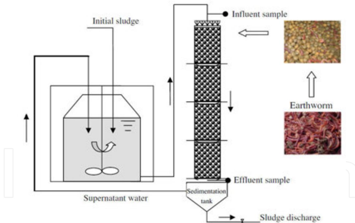
Figure 46. Schematic diagram of a vermifilter [24].
