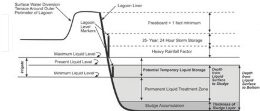
Figure 18. Anaerobic wastewater treatment lagoon [12].
