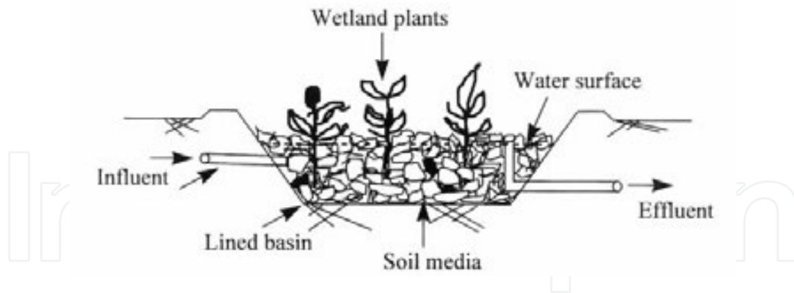
Figure 42. Sub-surface flow system [18].
