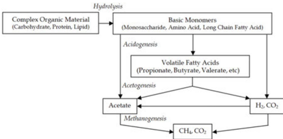
Figure 6. Steps of the anaerobic digestion process [8].
