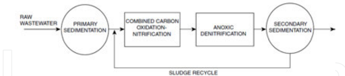
Figure 38. Nitrification/denitrification system for biological removal of nitrogen [3].
