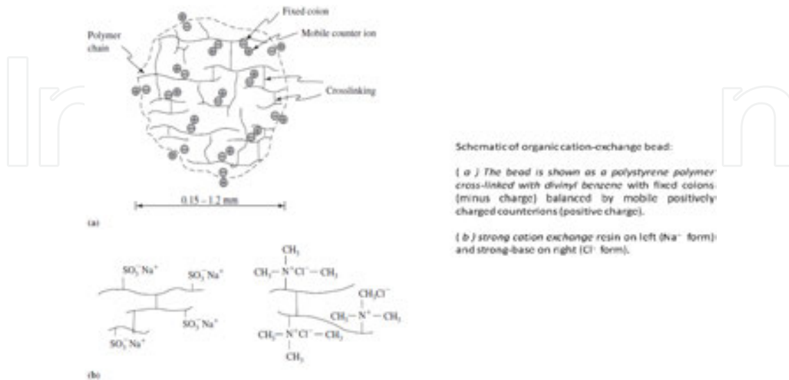
Figure 53. Schematic illustration of organic cation-exchange bead [34].
