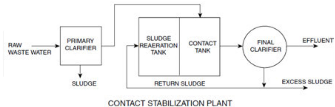
Figure 26. Contact stabilization plant [3].
