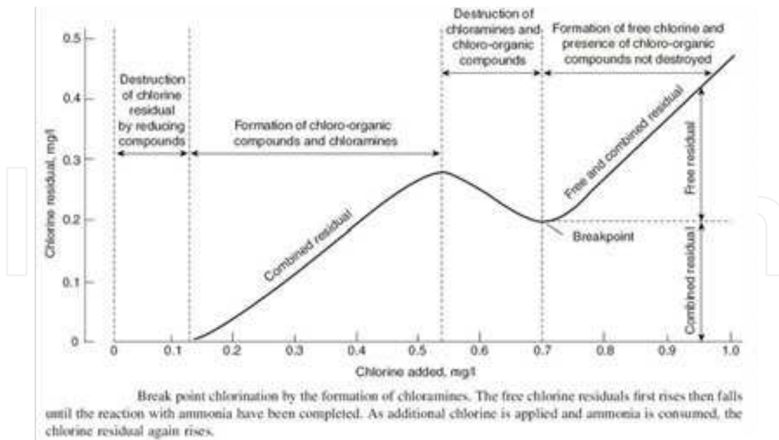
Figure 51. Chlorination curve [3].
