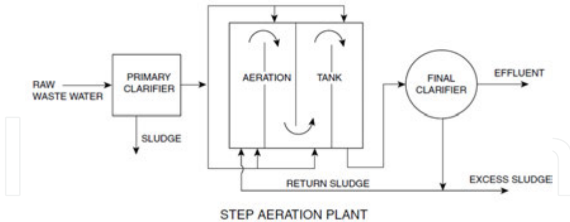
Figure 27. Step aeration plant [3].
