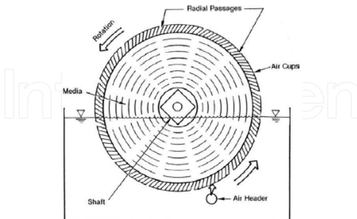
Figure 33. Schematic diagram of air-drive RBC [2].
