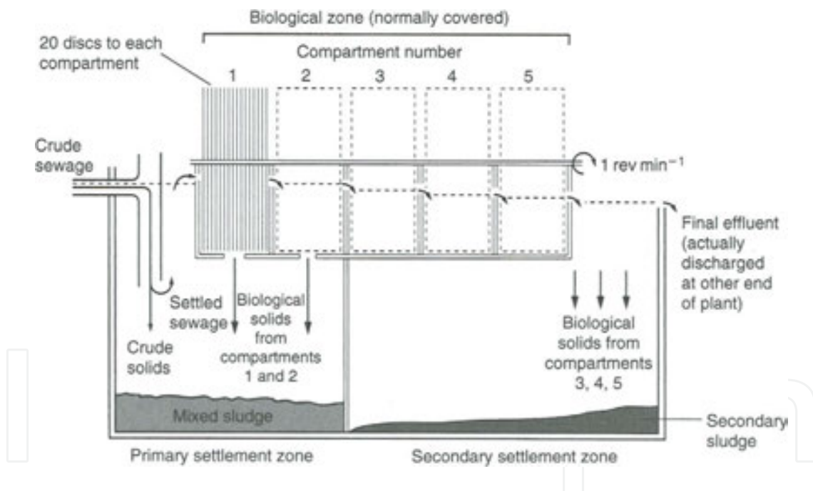
Figure 35. RBC system [1].
