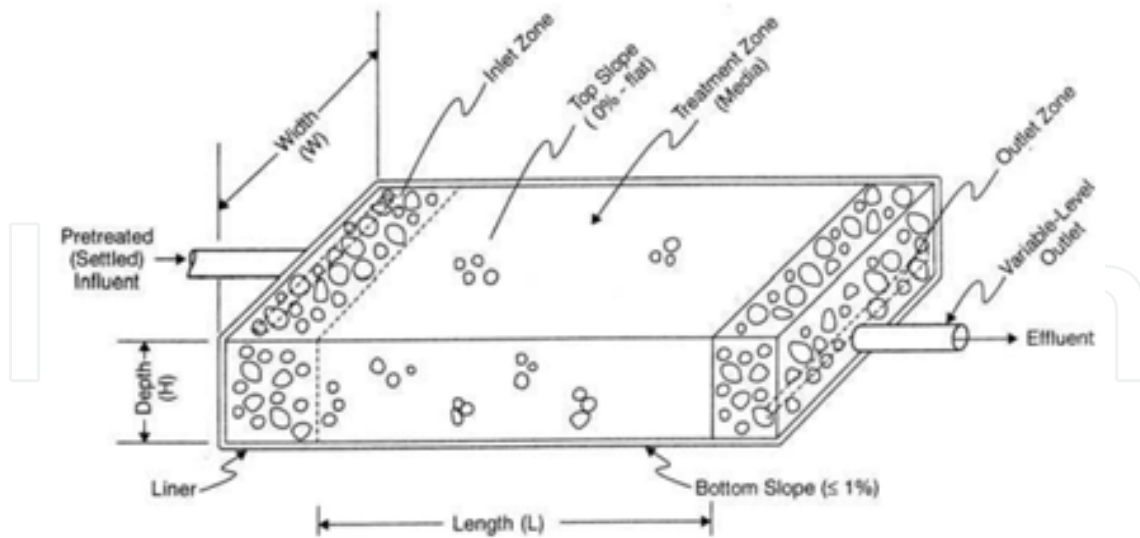
Figure 44. Components of a vegetated submerged bed system [2].
