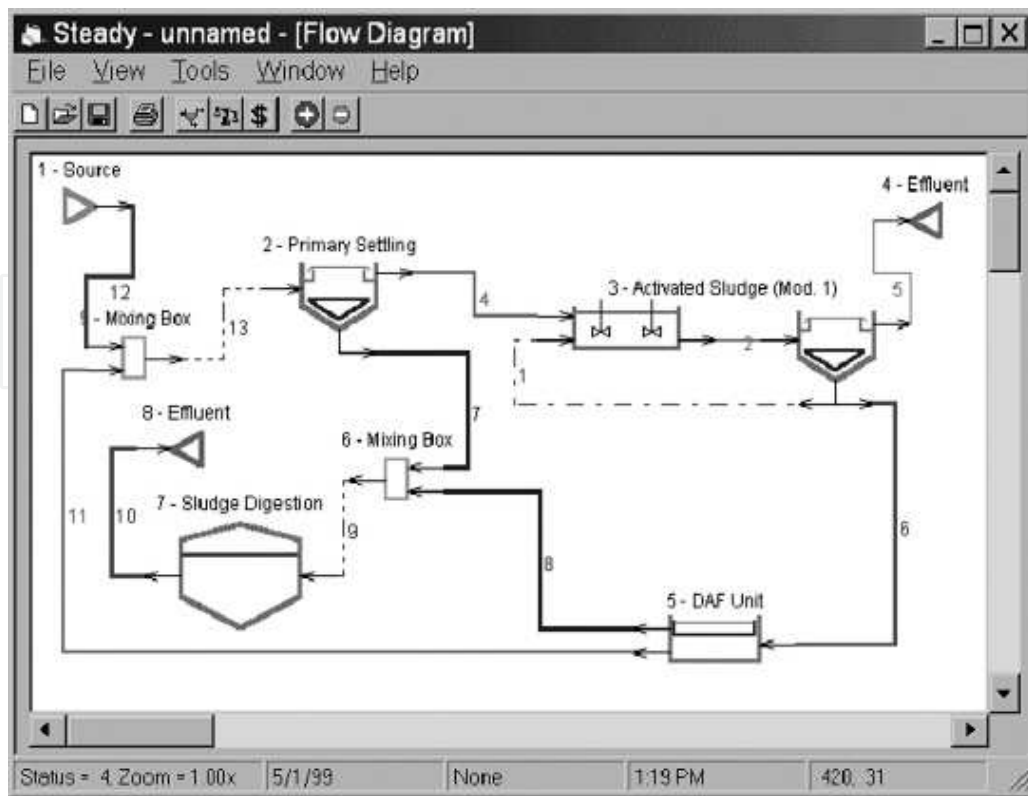
Figure 57. Screenshot of the STEADY program [3].
