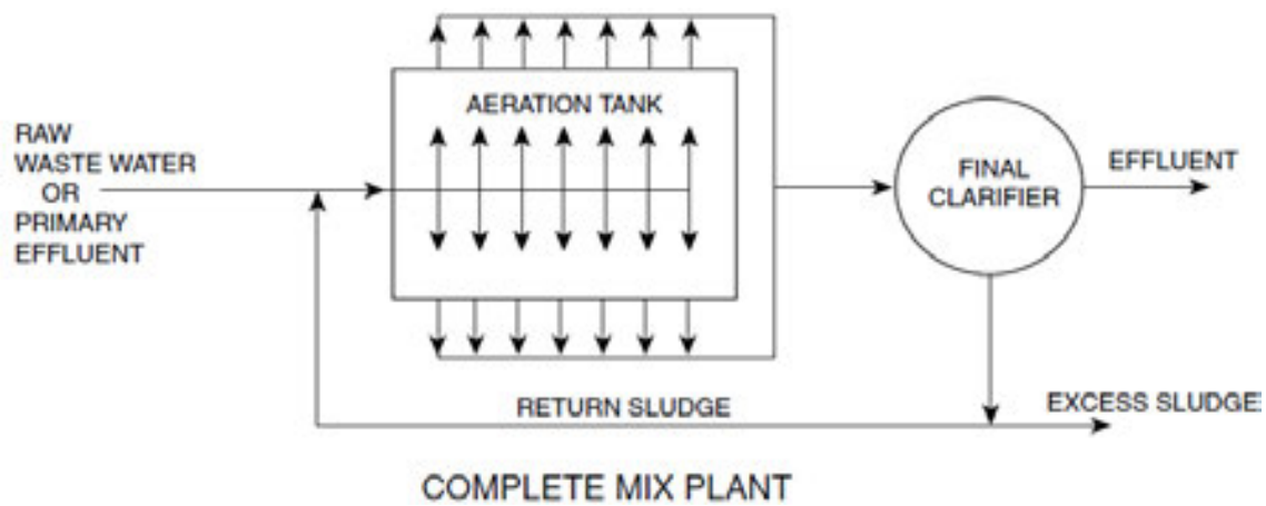
Figure 25. Complete mix plant [3].
