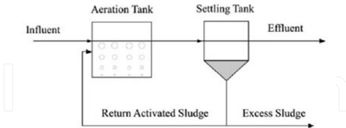
Figure 23. Activated sludge [15].
