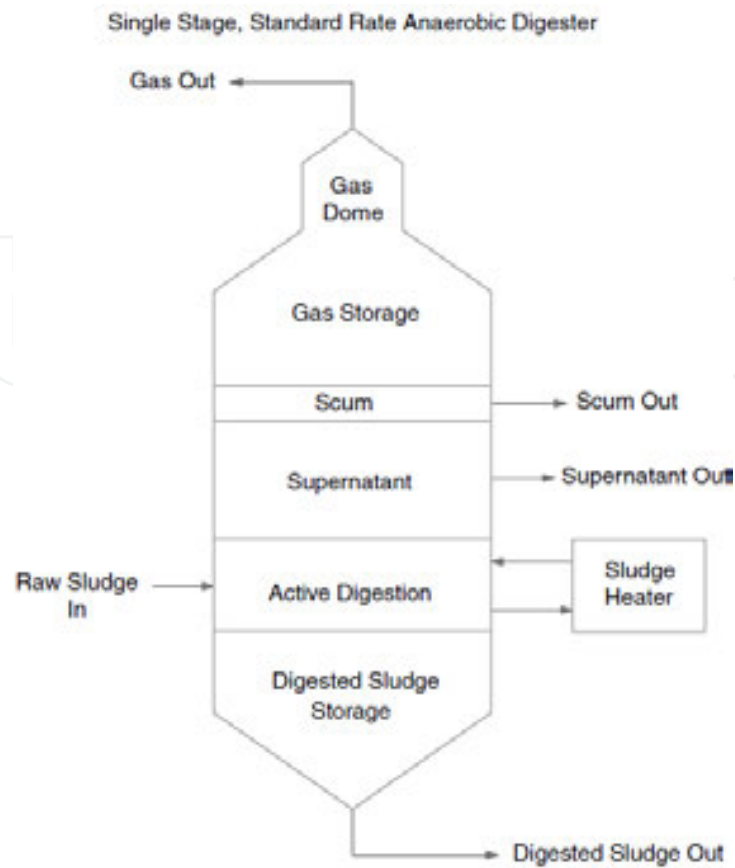
Figure 9. Single-stage conventional anaerobic digester [3].
