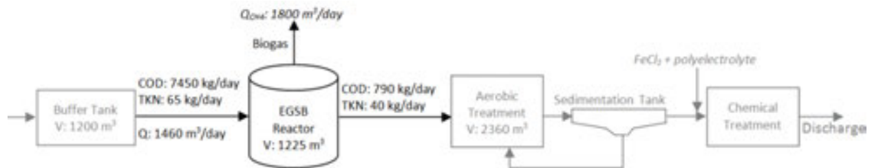
Figure 14. Wastewater treatment plant for corn processing industry [8].
