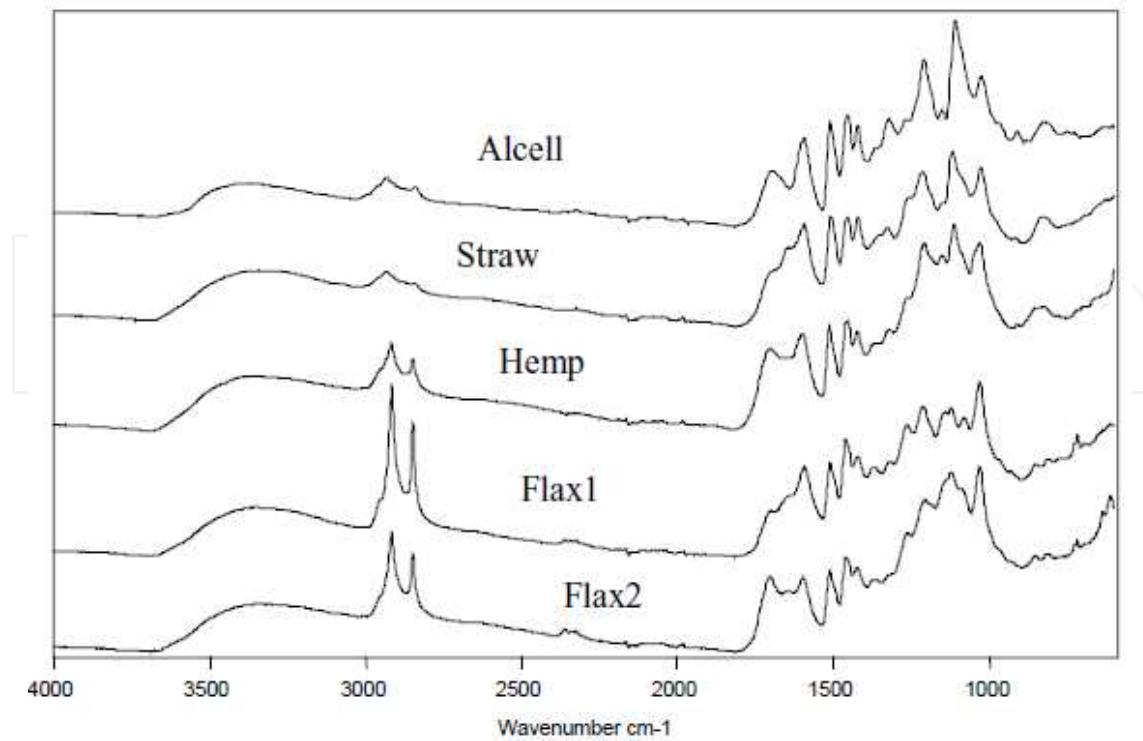
Figure 2. FTIR spectra of lignin from different substrates [52].
