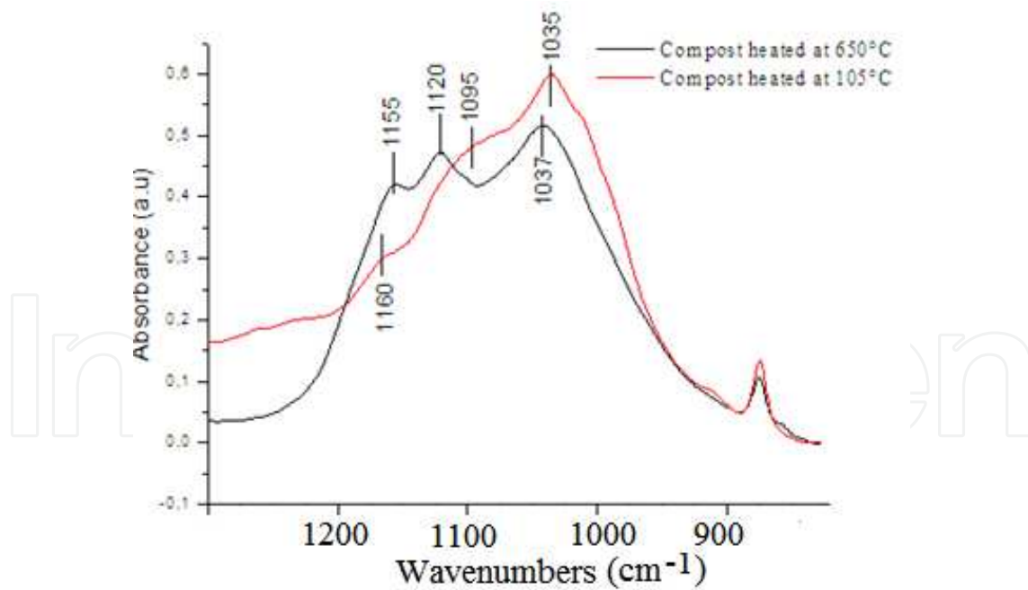
Figure 3. FTIR spectra before and after calcination of compost.
