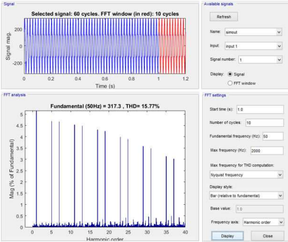
Fourier Analysis of Harmonic Distortion at 0.4kV Bus
