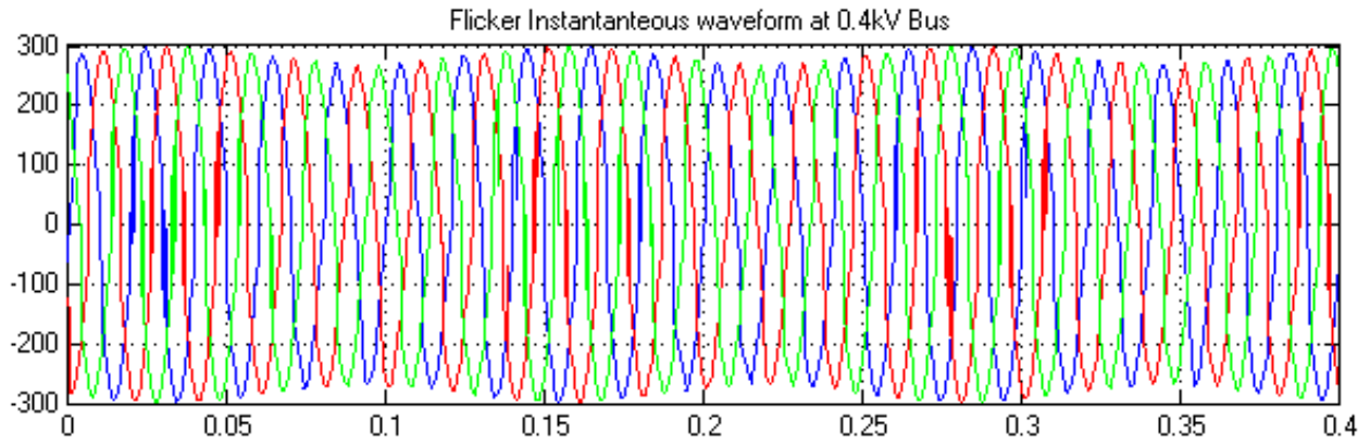
Figure 30. Flicker waveform disturbance caused by electric arc furnace at 0.4 kV bus.
