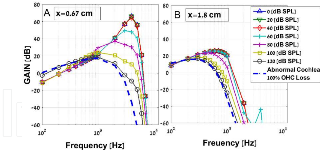
Figure 3. Derivation of the basilar membrane gain ( |\xi_{\text{bm}}(x_0)| / P_0 ) as a function of input frequency at two locations along the cochlear partition: x = 0.67 \text{ cm} from the stapes (A) and x = 1.8 \text{ cm} from the stapes (B). Each solid line represents a different input level and a normal cochlea ( \gamma_{\text{ohc}} = 0.5 ). The broken line represents a damaged cochlea ( \gamma_{\text{ohc}} = 0 ). A similar gain was obtained for all input levels.
