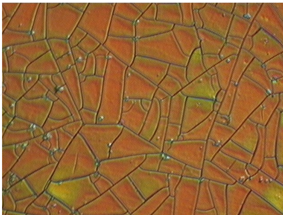
Figure 2. Optical Micrograph of an electrodeposited cerium oxide film on stainless steel. 800x magnification. (from T. Golden).
