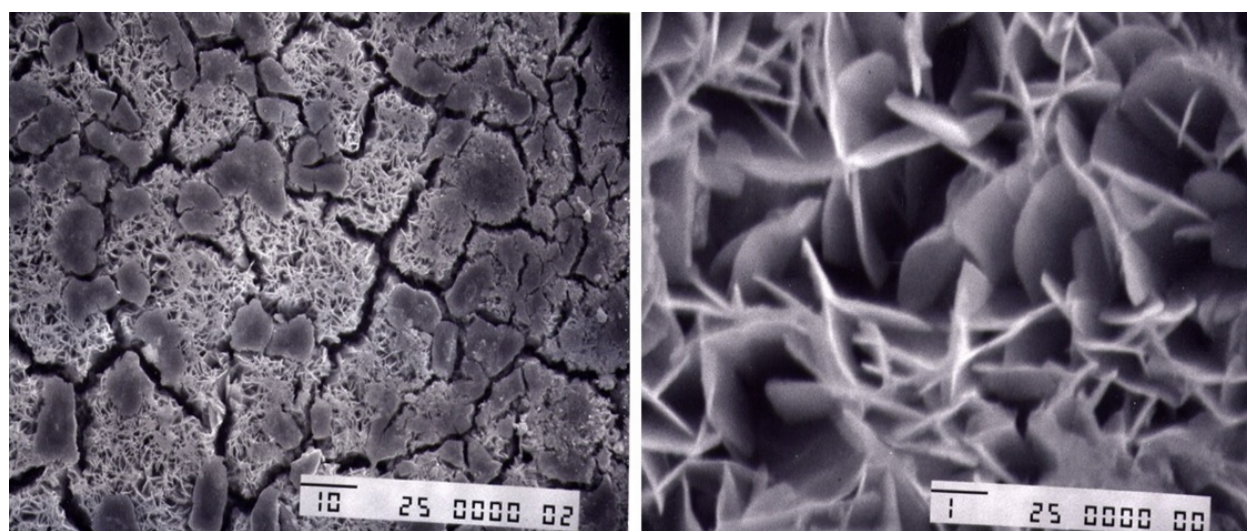
Figure 9. SEM images of Pr 6 O 11 film obtained by cathodic electrodeposition on stainless steel in an electrolyte system composed of 0.1M Pr(NO 3 ) 3 and 0.1M NH 4 NO 3 solution, j = 0.8 \text{ mA/cm}^2 , T = 25 \text{ }^\circ\text{C} , and after sintering at 600 °C for 1 h; (left) magnification 1000. (T. Golden); (right) magnification 10000.
