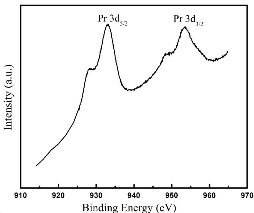
Figure 8. High-resolution XPS spectra of Pr 3d core level showing the spin-orbit splitting of the 3d level.
