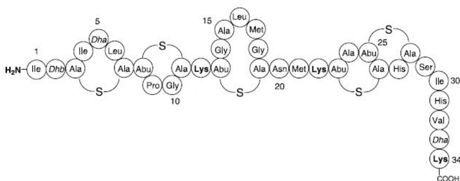
Figure 1. Schematic representation of the primary structure of nisin produced by L. lactis subsp. lactis ATCC 11454. Ala-Ala-S represents lanthionine; Abu-S-Ala- \beta -methyl, lanthionine, dehydroalanine Dha, and Dhb dehydrobutirine [19].
