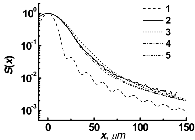
Figure 15. Spot-scan profile S(x) in the D-2 detector measured at V_g=0.95 V (curve 2) in comparison with the profiles S(x) calculated by the 2D diffusion model with k_{ph}=20, 40, and 60 (curves 3, 4, and 5, respectively). Curve 1 is the distribution of the IR radiation intensity.
