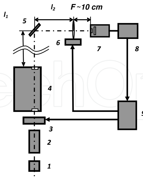
Figure 9. Experimental setup: 1 – glöbar, 2 – collimator, 3 – PC-controlled shutter, 4 – monochromator, 5 – deflecting mirror, 6 – focusing lens mounted on a motorized XYZ stage, 7 – cryostat with the mounted FPA detector, 8 – electronic equipment controlling ROIC operation and measuring the photoelectric signals, 9 – personal computer.
