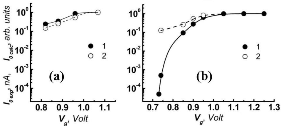
Figure 17. Comparison of the photocurrent values I_{o\ exp} evaluated from the measured voltage photosignals \Delta V(I) for the spot-centered diode with the photocurrent values I_{o\ calc} calculated by the 2D diffusion model (2) for the D-1 (a) and D-2 (b) detectors. The data for D-2 were normalized to make them refer to the same IR radiation intensity in the illumination spot.
