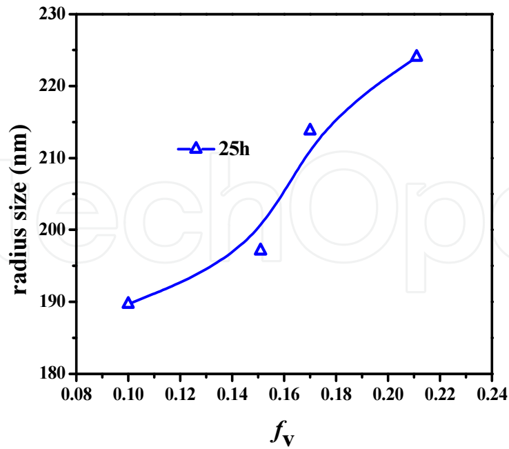
Figure 20. Radius as a function of volume fraction of precipitates.
