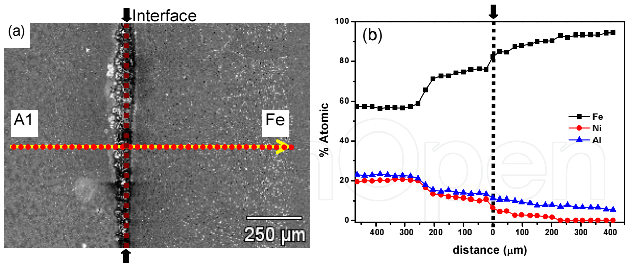
Figure 15. SEM micrograph of the (a) diffusion couple and (b) EDS chemical composition.
