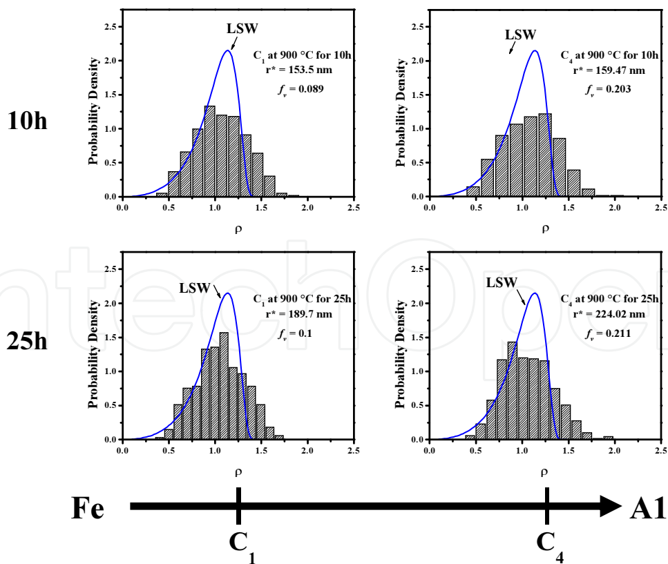
Figure 21. Precipitates size distribution for different compositions.
