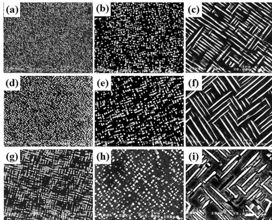
Figure 7. SEM micrographs of the precipitation evolution for the Fe-10wt.%Ni-15wt.%Al-1wt.%Cu alloy aged at (a,d,g) 750, (b,e,h) 850 and (c,f,i) 950 °C for 25, 75 and 200 h, respectively.
