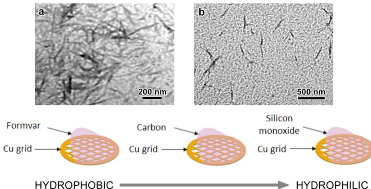
Figure 4. Comparison of never-dried CNCs at pH 5-6 on different types of supporting films: a) formvar; b) silicon monoxide (reproduced from [78] by permission of the KTH Royal Institute of Technology).
