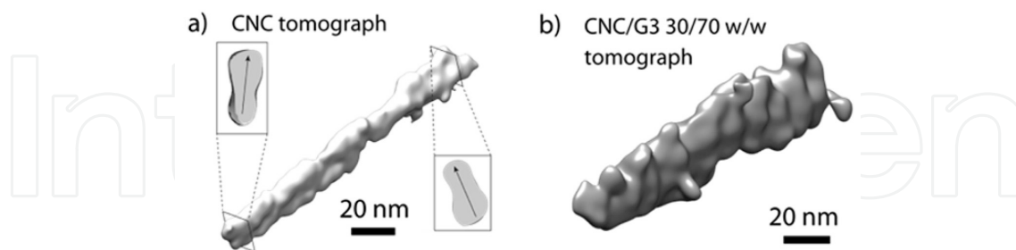
Figure 15. Electron tomography reconstitution of initial (a) and dendronized (b) polymer-wrapped cotton CNCs (reprinted with permission from [62]. Copyright 2014 American Chemical Society).
