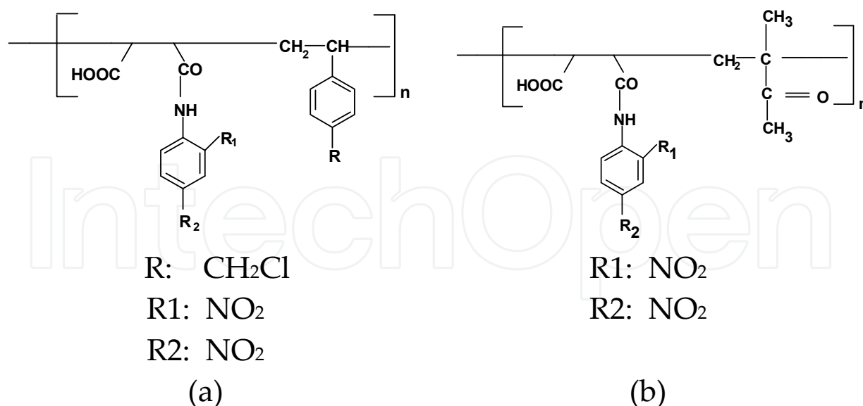
Figure 28: Selected copolymers: P1: MA-CMS-DNA (a); P2: MA-MMA-DNA (b)
