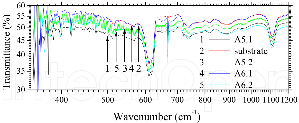
Figure 22. FTIR spectra of A5 and A6 thin films deposited at different nitrogen pressure: 0.05 torr A5.1 and A6.1; 0.2 torr A5.2 and A6.2 [29].
