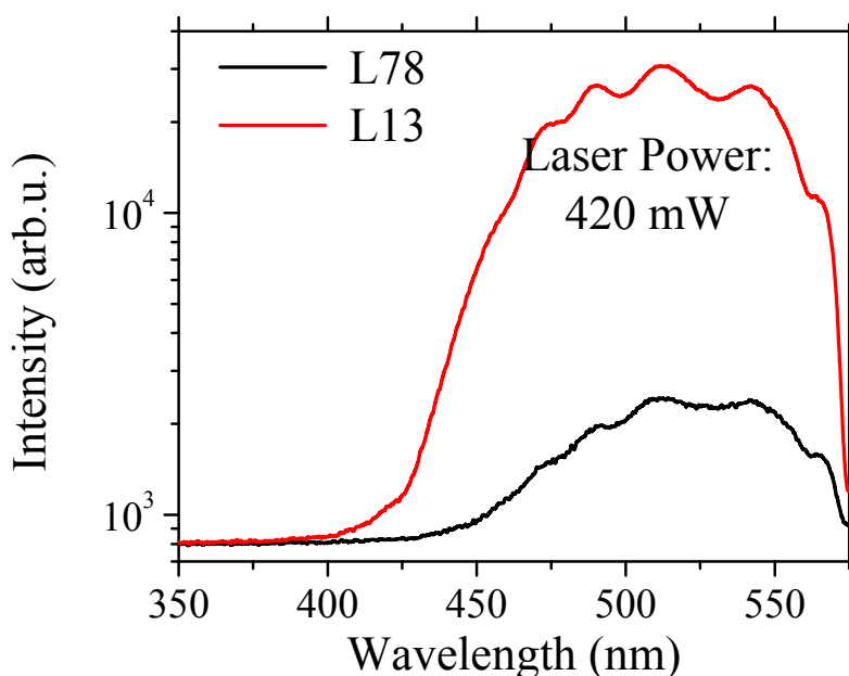
Figure 14. Fluorescence emission induced by two-photon absorption in oligomers L78 and L13 thin films deposited by vacuum evaporation on Si [31].
