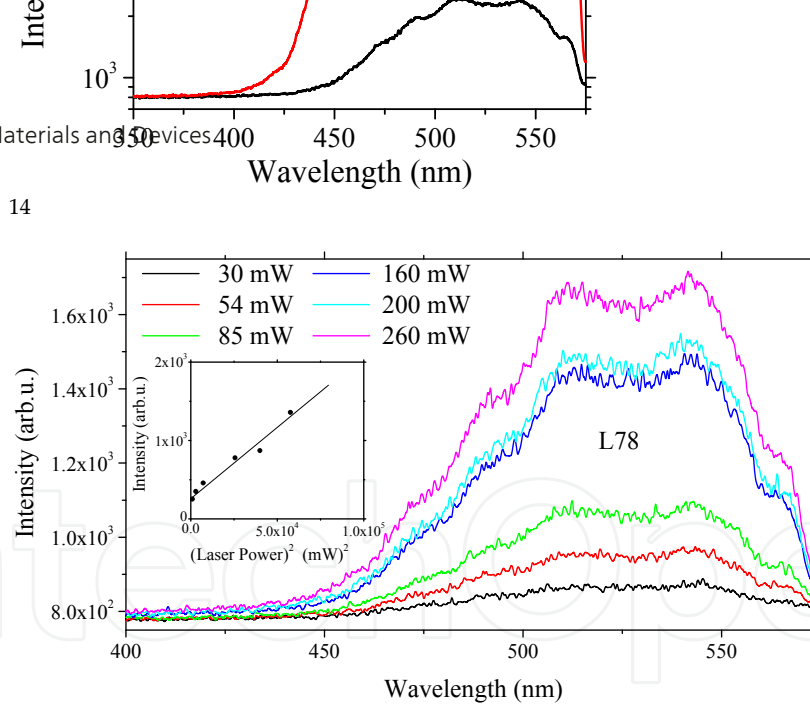
Figure 15. Dependence of TPF on laser power for L78 films deposited by vacuum evaporation on Si [31].
