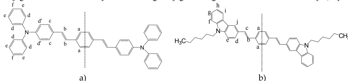
Figure 7: Chemical structures of the oligomers L78: 1,4-bis[4-(N,N'-diphenylamino)phenylvinyl] benzene (a); L13: 3,3'-bis(N-hexylcarbazole)vinylbenzene (b) [31].
