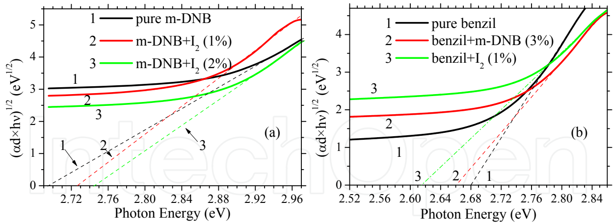
3 Figure 3. Tauc plots for: pure and doped m-DNB (a); pure and doped Bz (b) [19].
